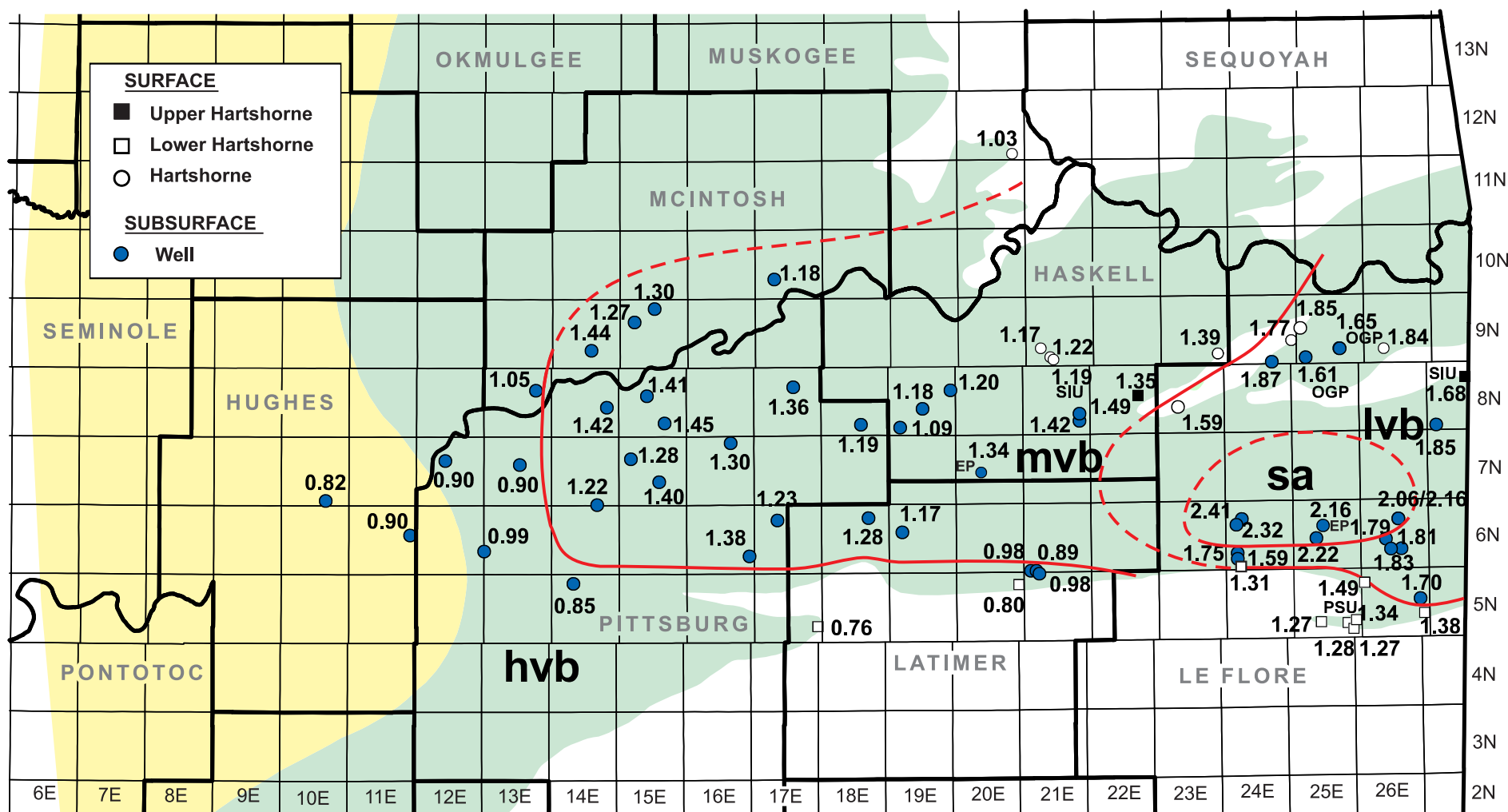
Preliminary coal rank map of Arkoma Basin based on mean maximum vitrinite reflectance of Hartshorne coal samples (hvb = high volatile bituminous; mvb = medium volatile bituminous; lvb = low volatile bituminous; sa = semianthracite). Data by Brian Cardott, Oklahoma Geological Survey, unless specified otherwise. Additional data from OGP Operating (OGP), The Pennsylvania State University (PSU), Southern Illinois University at Carbondale (SIU), and Pratt and others (2004; El Paso cores, EP). Revised 5/2009.
