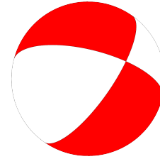
Fault Plane Solution
