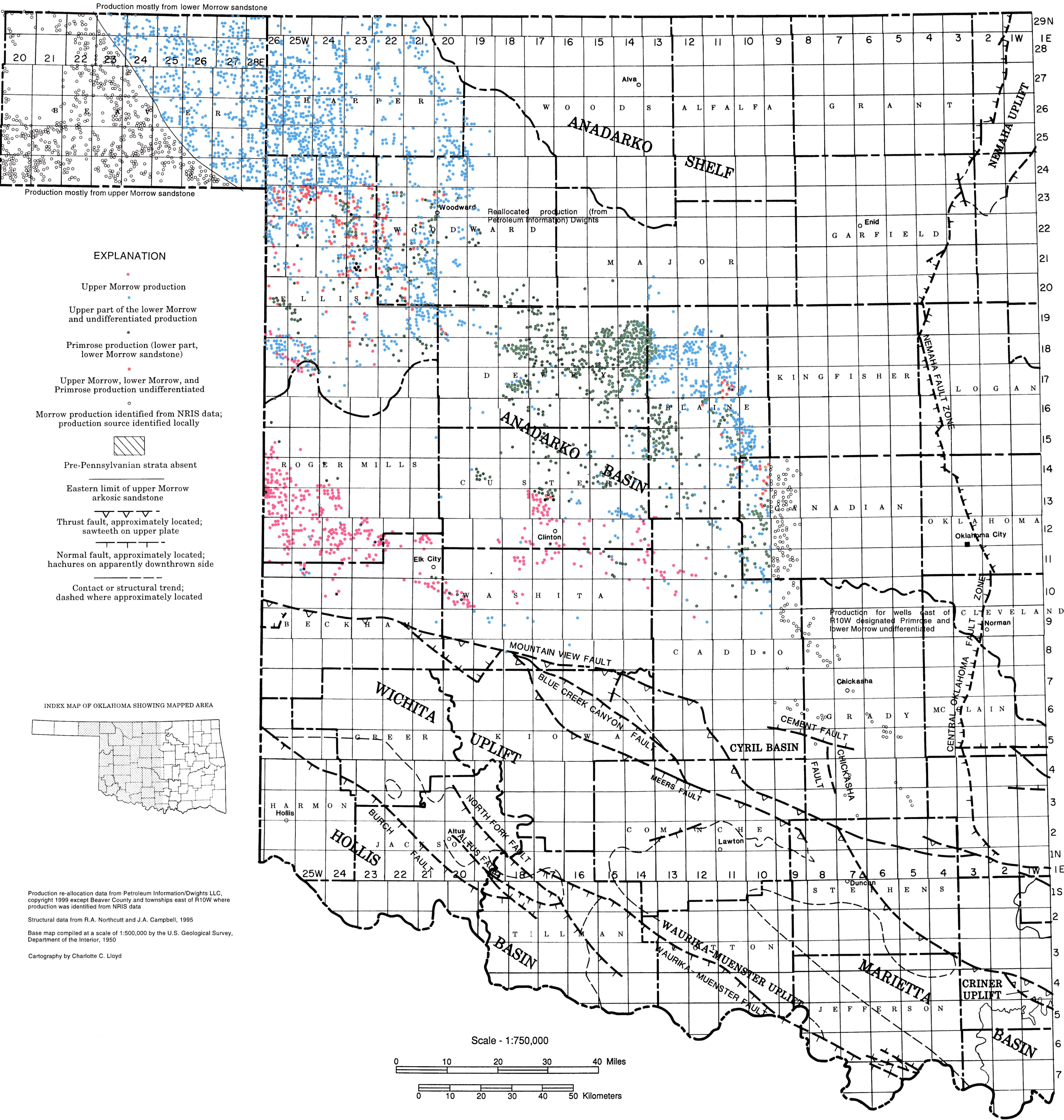
GENERALIZED MAP SHOWING WELLS WITH PRODUCTION FROM THE MORROW AND PRIMROSE SANDSTONES IN THE ANADARKO BASIN AND SHELF OF OKLAHOMA
