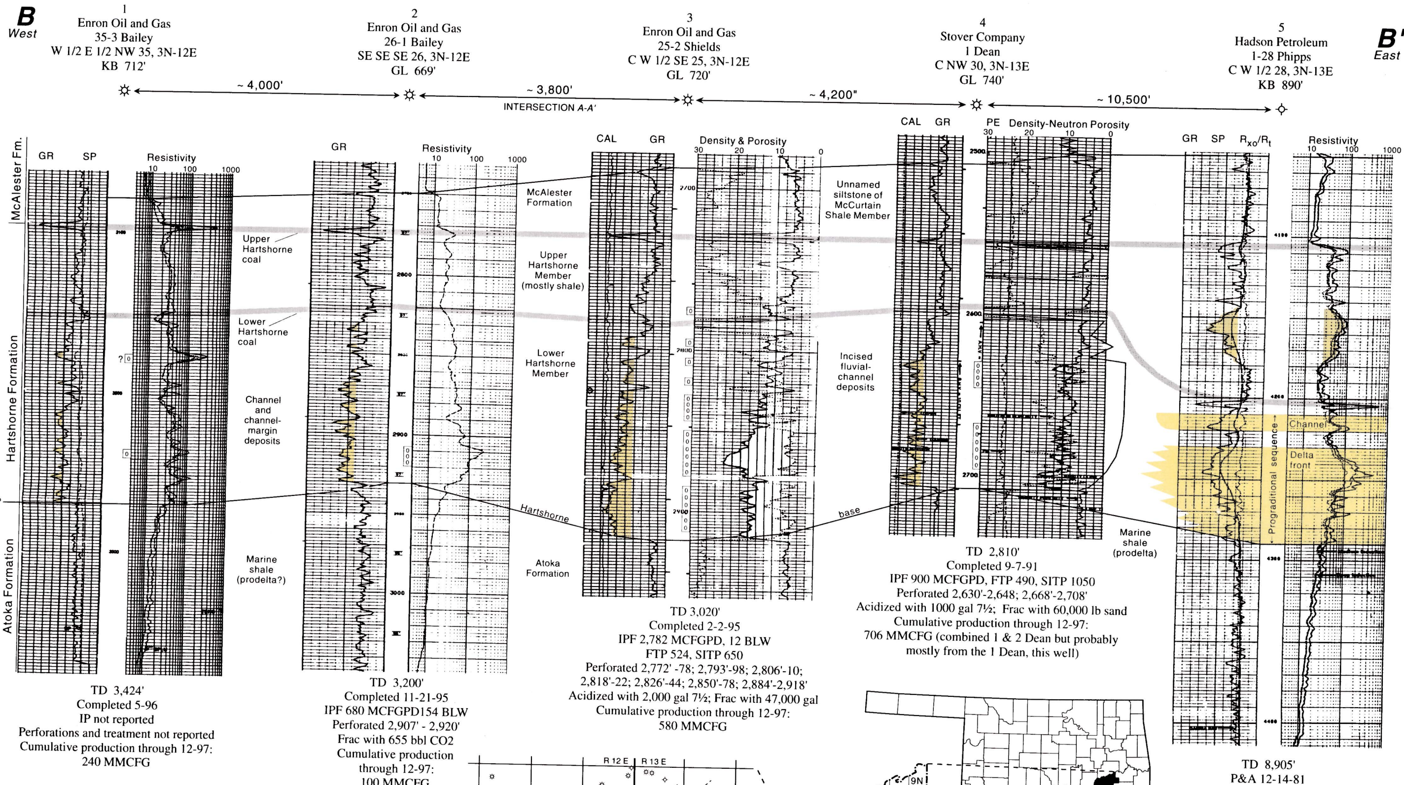
Figure 25. Stratigraphic cross section B-B' and index map, Kiowa NW field, southwest Pittsburg County, Oklahoma. Datum: top of Upper Hartshorne coal.
