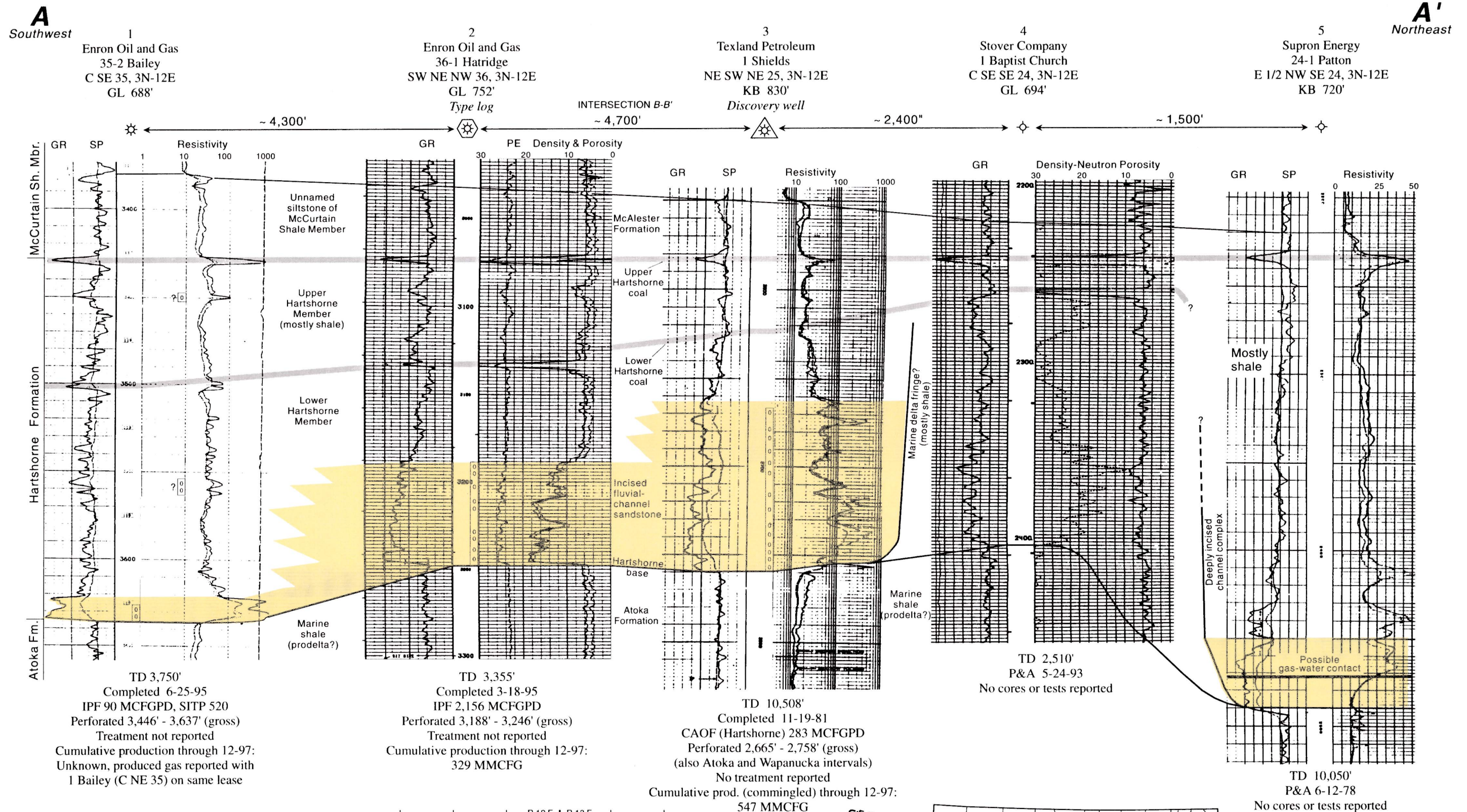
Figure 24. Stratigraphic cross section A-A' and index map, Kiowa NW field, southwest Pittsburg County, Oklahoma. Datum: top of Upper Hartshorne coal. Vertical scale, 1 in. = ~60 ft; no horizontal scale. GR = gamma ray, SP = spontaneous potential, CAL = caliper, PE = photoelectric, R_{x0} = resistivity of flushed zone, R_t = resistivity of uninvaded zone ("true" resistivity).
