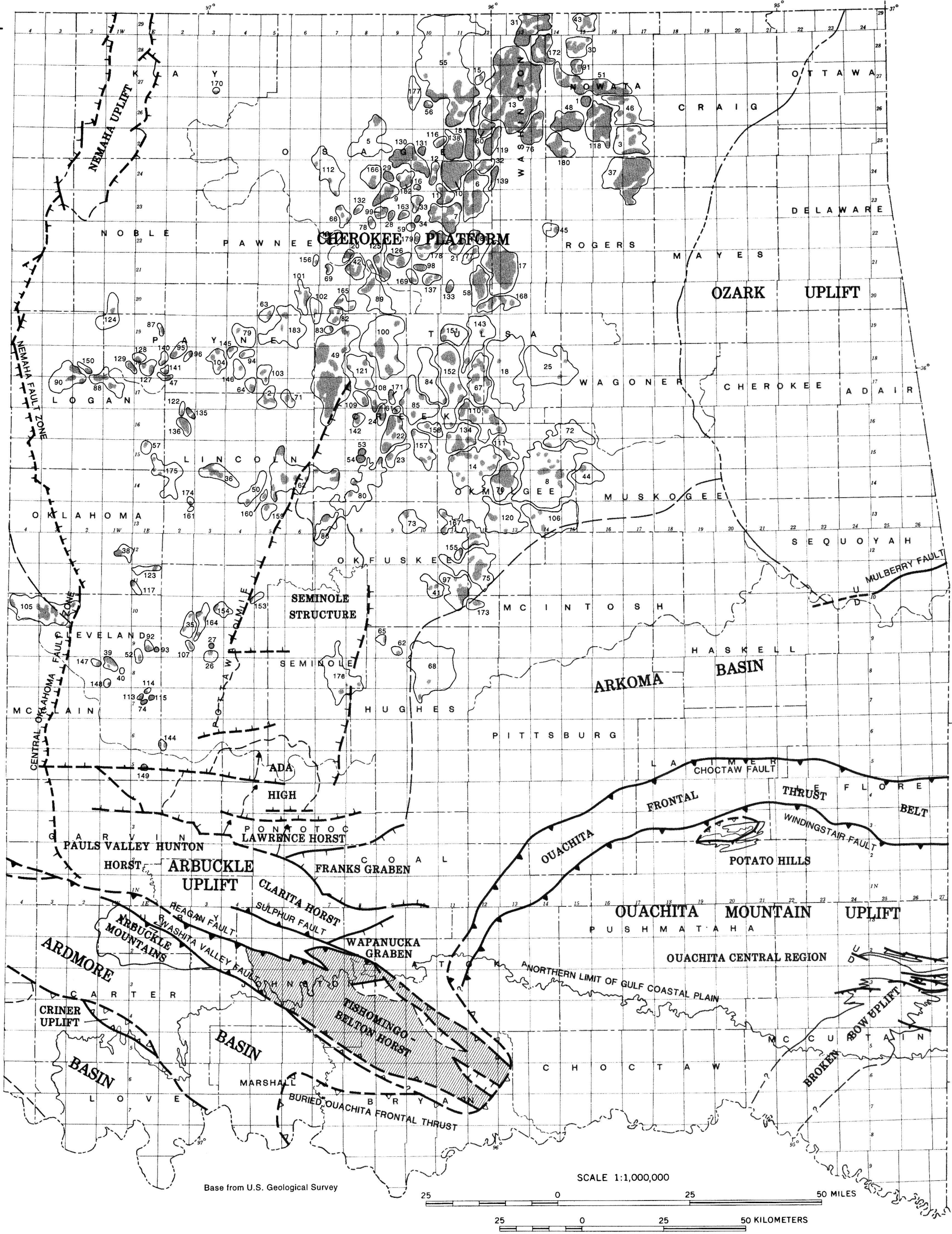
FLUVIAL-DOMINATED DELTAIC (FDD) OIL RESERVOIRS IN OKLAHOMA: THE BARTLESVILLE SANDSTONE PLAY MAP OF FIELDS WITH OIL PRODUCTION FROM THE BARTLESVILLE SANDSTONE
