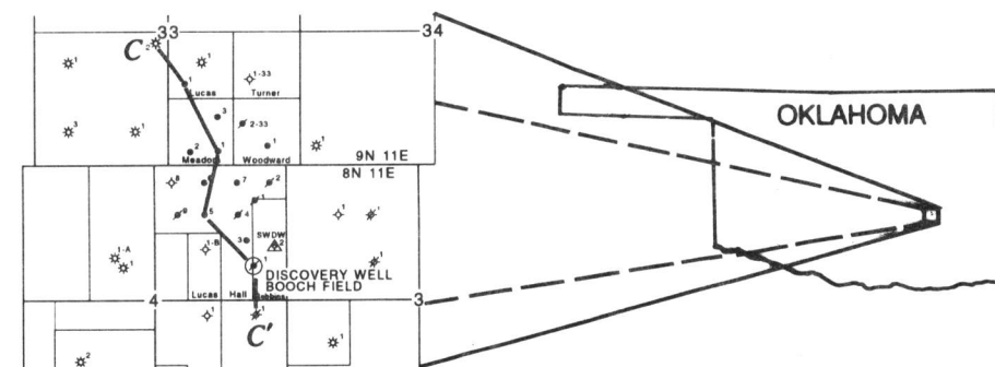
INDEX MAP SHOWING LOCATION OF CROSS SECTION
