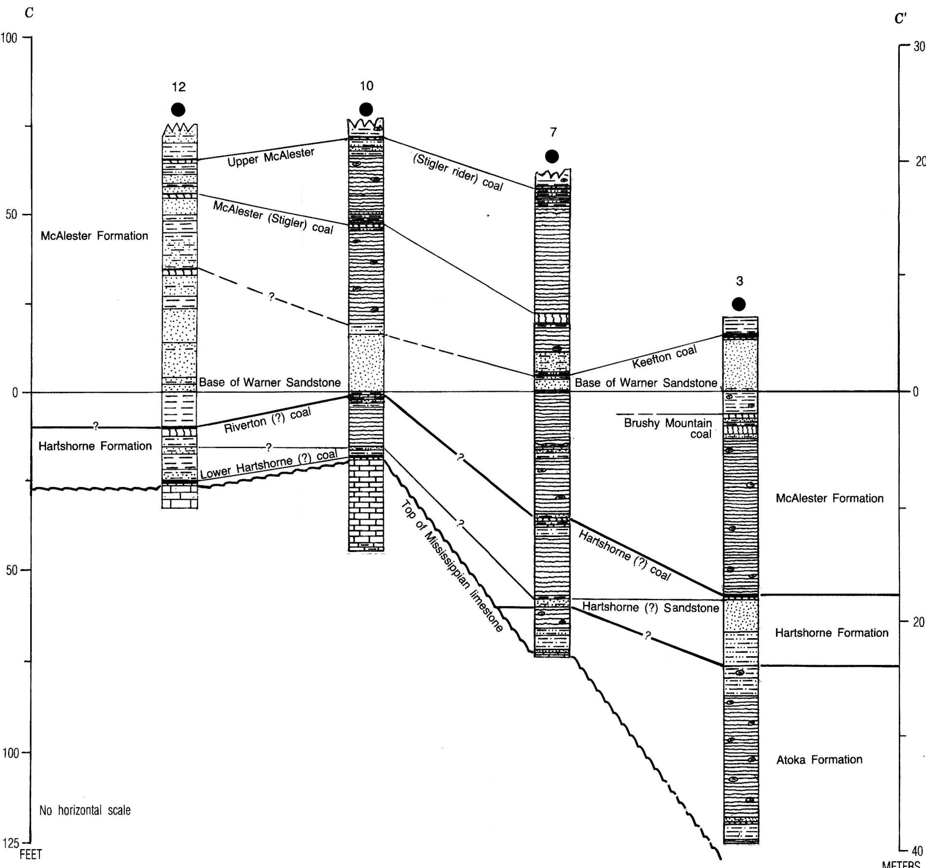
CROSS SECTIONS SHOWING ALTERNATIVE CORRELATIONS OF PENNSYLVANIAN UNITS BELOW THE WARNER SANDSTONE, NORTHEASTERN OKLAHOMA SHELF AREA
