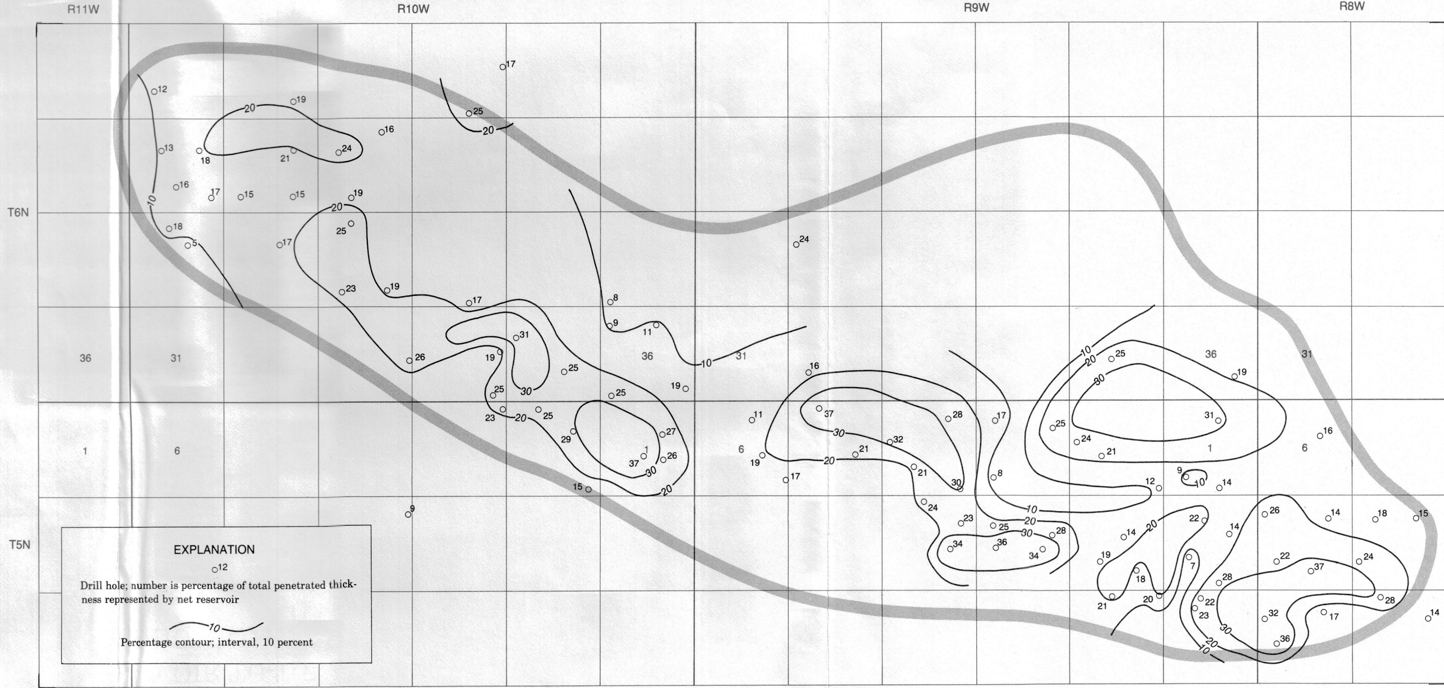
FIGURE D. MAP SHOWING NET RESERVOIR-TO-TOTAL-THICKNESS RATIO OF PENETRATED PRE-PERMIAN ROCKS
