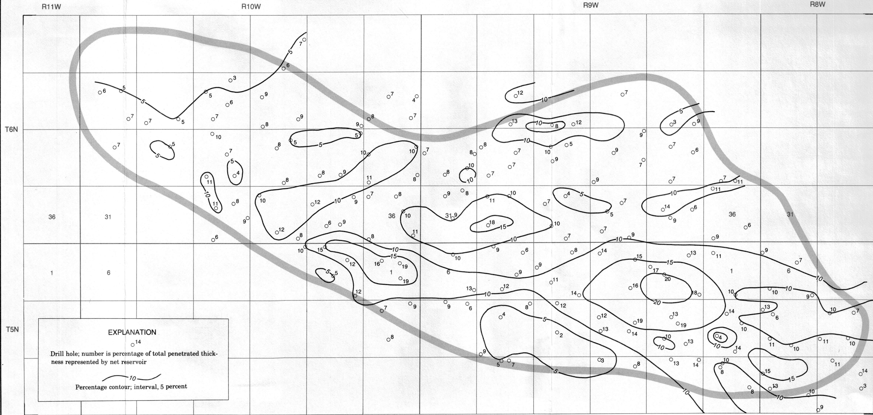
FIGURE B. MAP SHOWING NET RESERVOIR-TO-TOTAL-THICKNESS RATIO OF PENETRATED PERMIAN ROCKS
