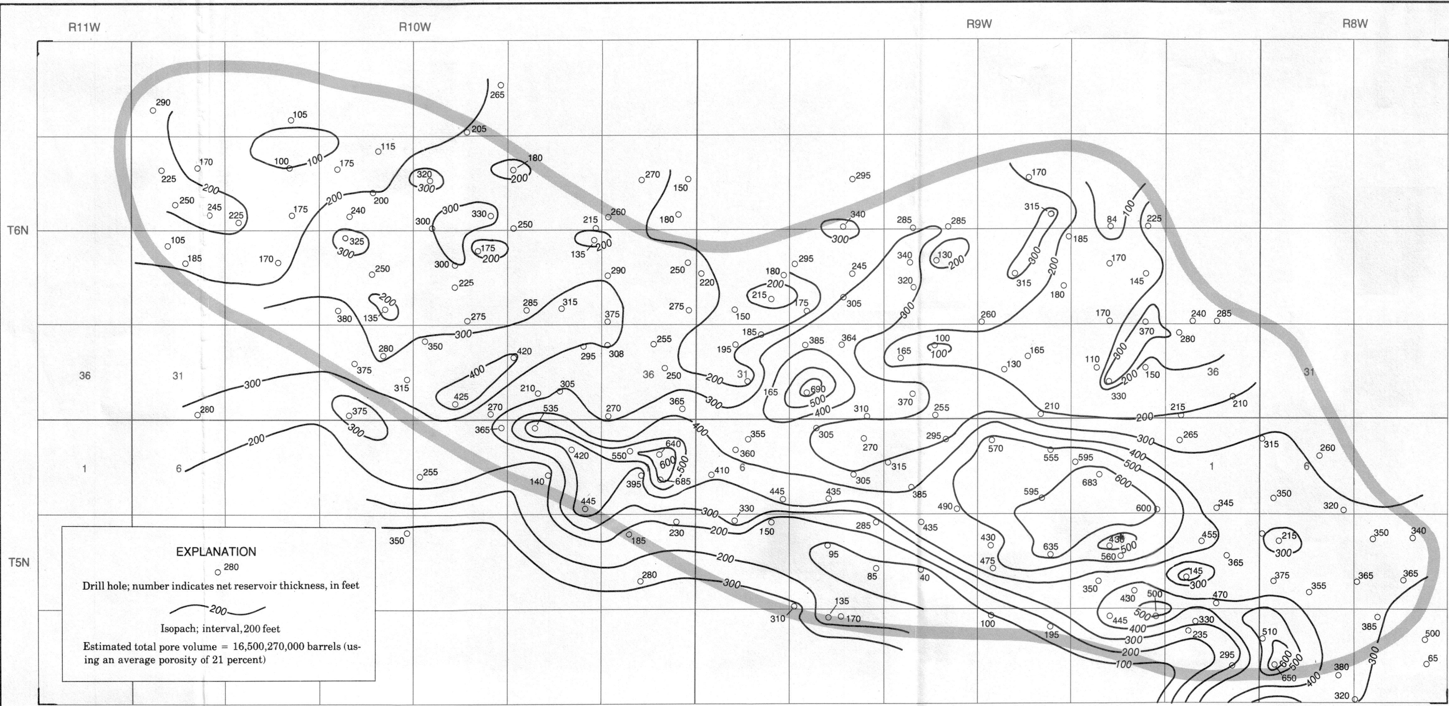
FIGURE A. MAP SHOWING NET RESERVOIR THICKNESS OF PENETRATED PERMIAN ROCKS
