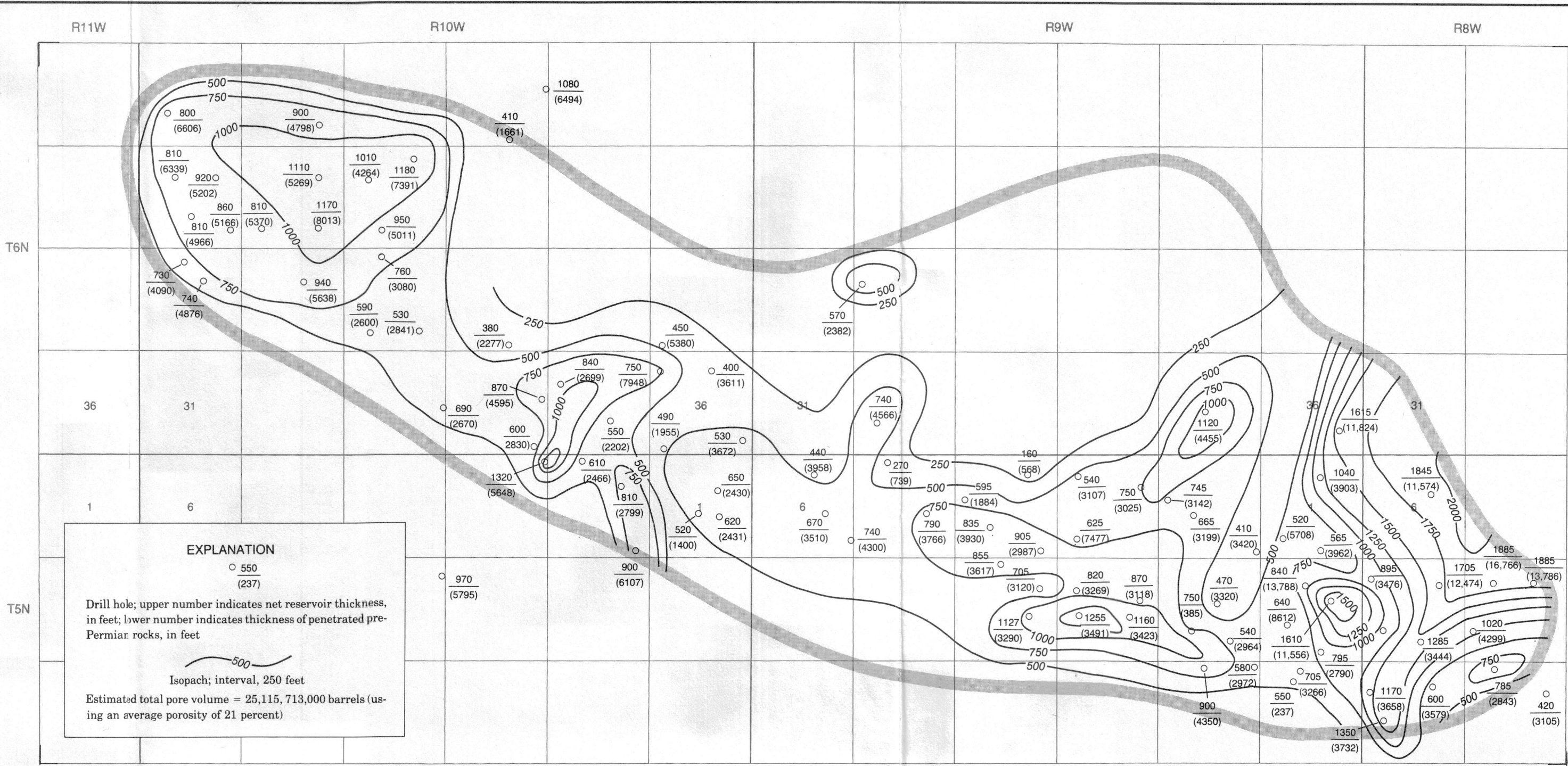
FIGURE C. MAP SHOWING NET RESERVOIR THICKNESS OF PENETRATED PRE-PERMIAN ROCKS
