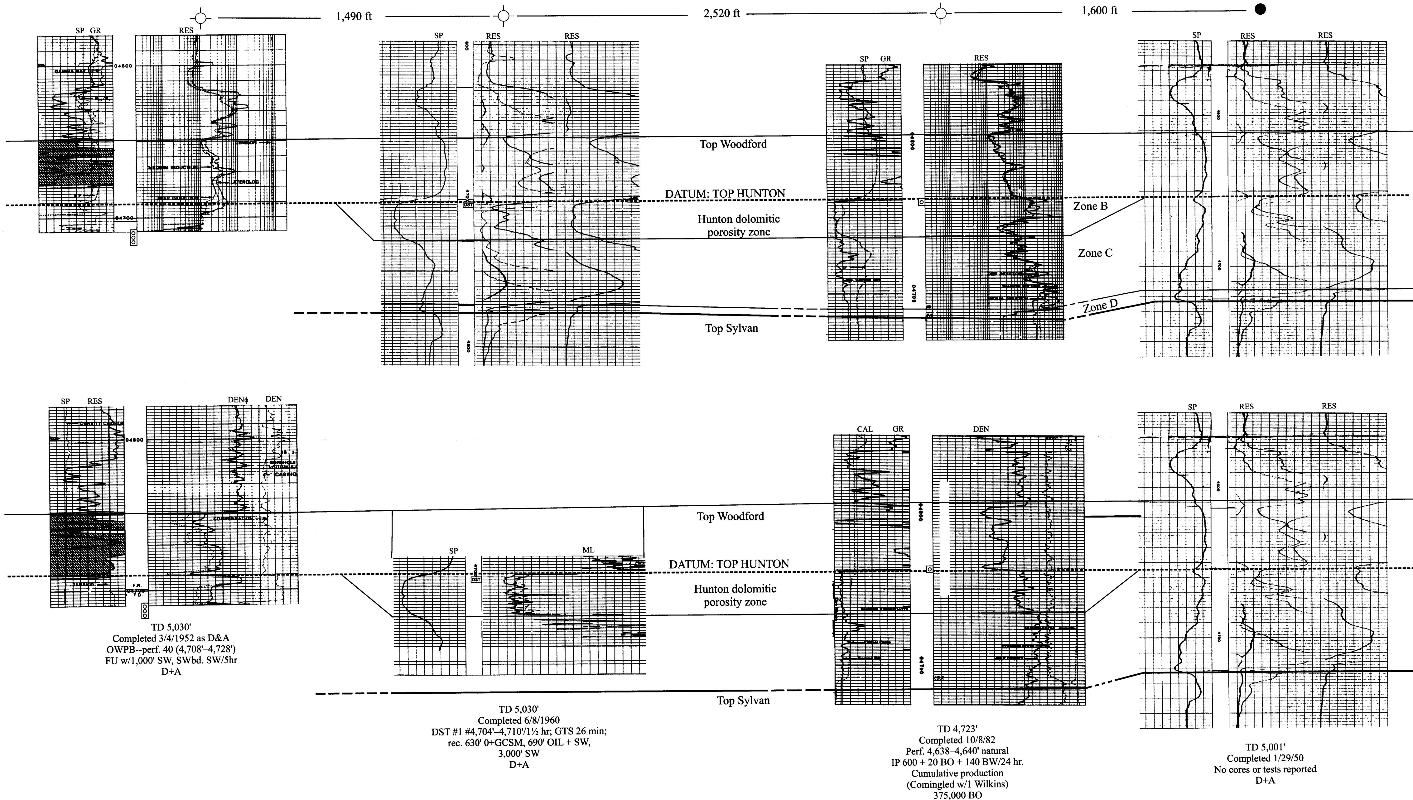
Figure 94. South-north stratigraphic cross section P-P' across Prairie Gem field, Lincoln County, Oklahoma. Line of section shown in Figures 93 and 122.
