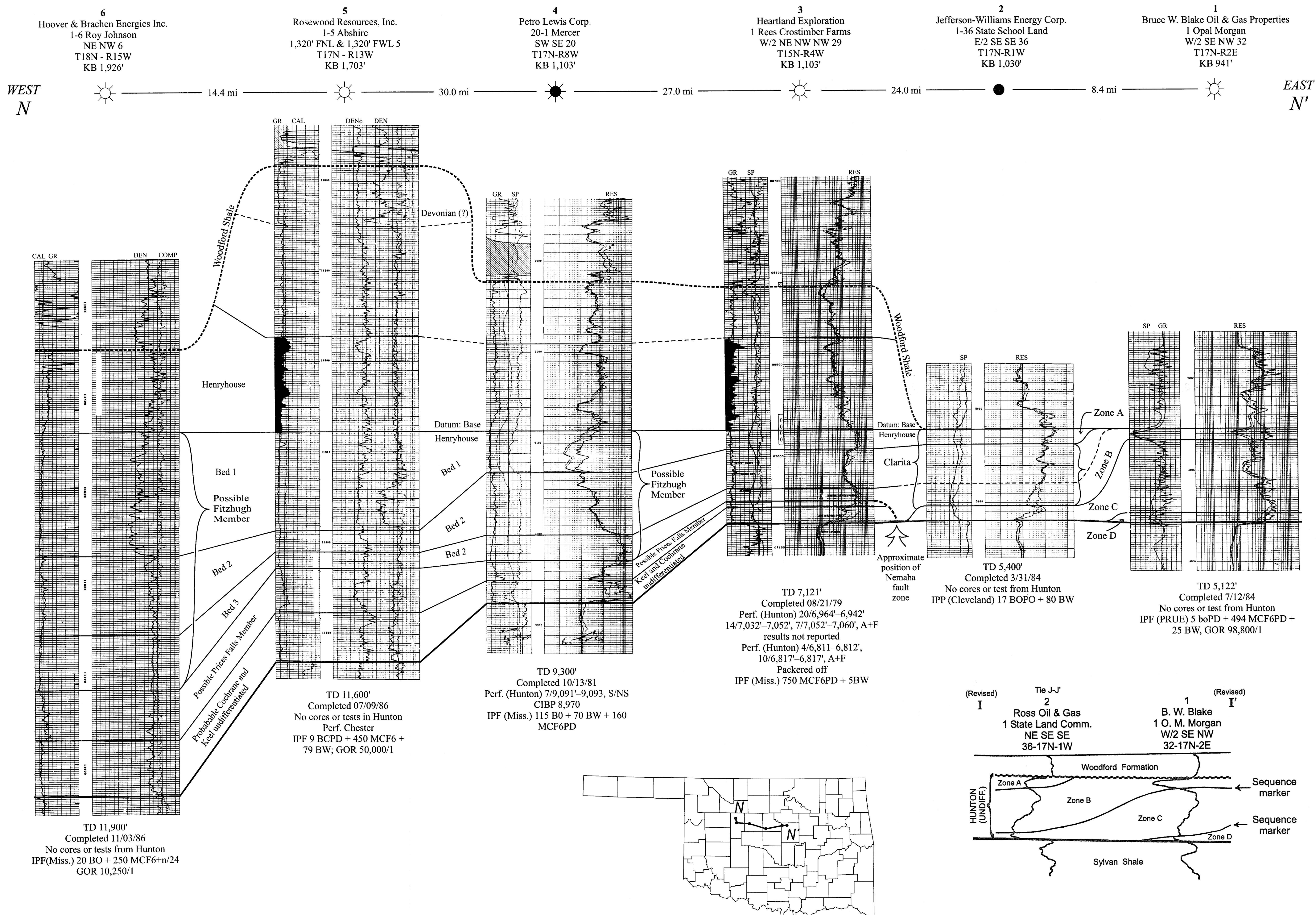
Figure 111. West-east stratigraphic cross section N-N'. Datum is base of Henryhouse Formation. Wells not horizontally to scale (Rottmann, 1993).
