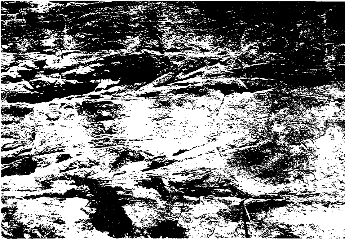
Figure 3. Two cross-bedded layers in the Rush Springs Sandstone in the canyon wall near Group Camp. These layers are in the lower, mostly non-cross-bedded part of the exposed sandstone. Note rock hammer (13 inches long) at lower right, for scale.
