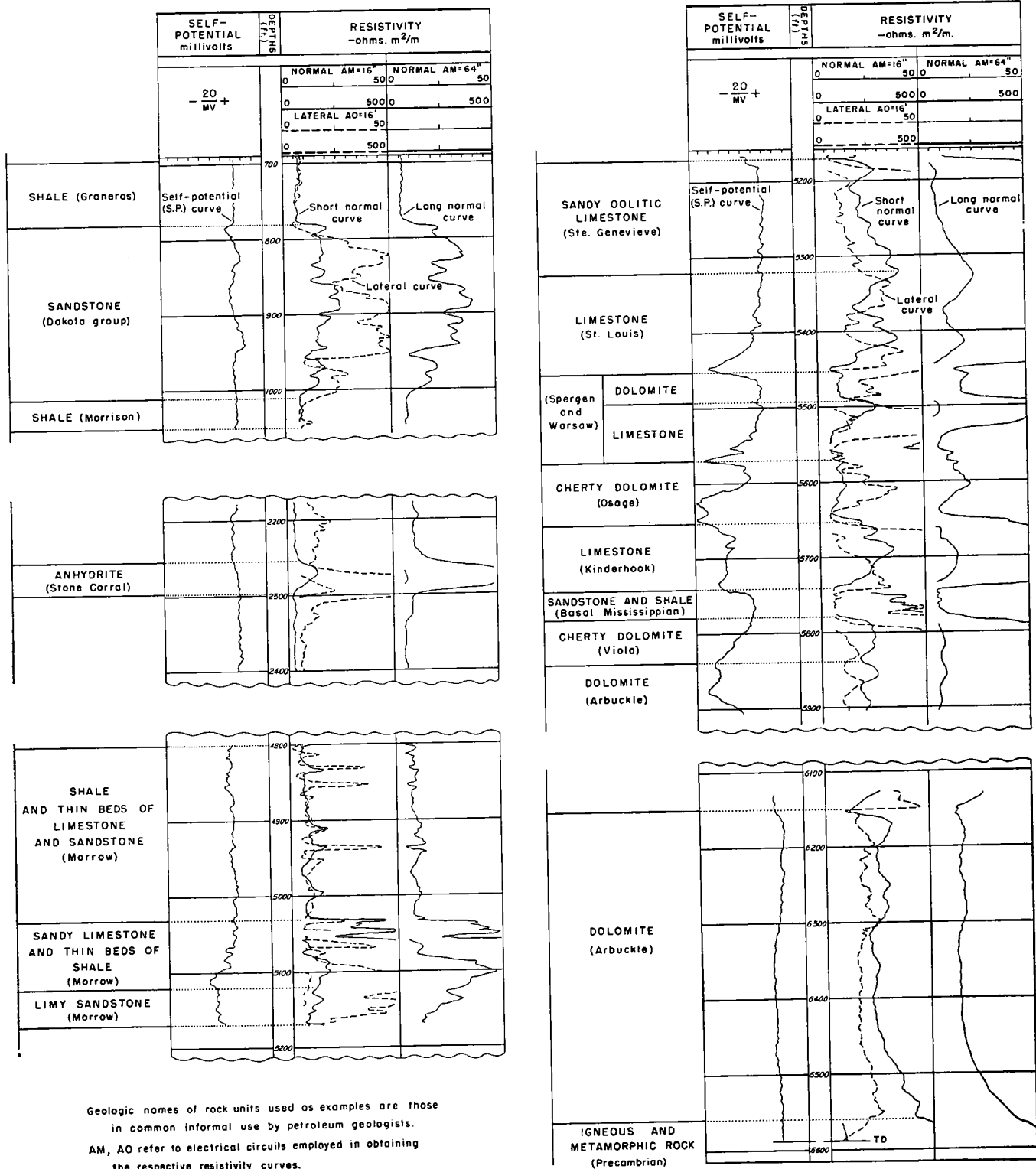
Fig. 3.- Examples of the expression of common lithologies by electric-log curves of wells in southeastern Colorado. Note that some dissimilar lithologies may have similar curves, and that detailed conclusions regarding lithology cannot be derived from the curves alone.
