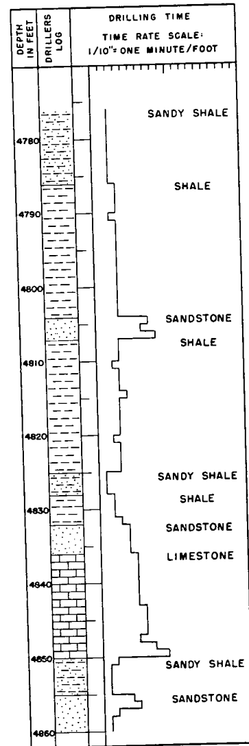
B. DRILLING-TIME AND DRILLERS LOG PLOTTED FROM DRILLER'S RECORDS.
