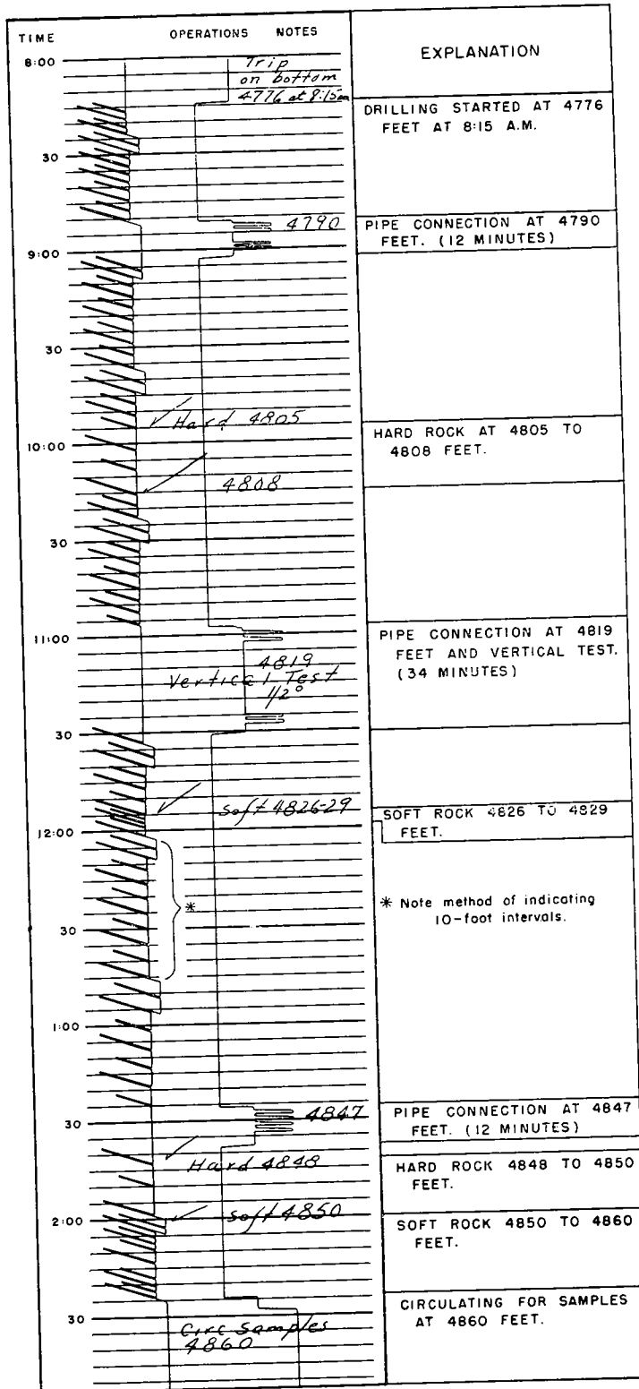
A. MECHANICALLY RECORDED DRILLING-TIME CHART WITH DRILLER'S NOTES. EXPLANATION AT RIGHT. (Adapted from Geograph.)
