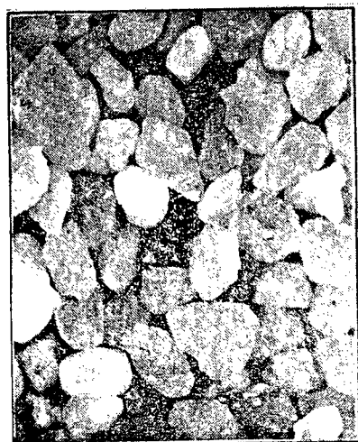
A. Very coarse sand (1-2 mm.), x 6.3
