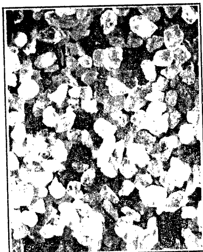
C. Fine sand (1/8-1/4mm.), x 18
