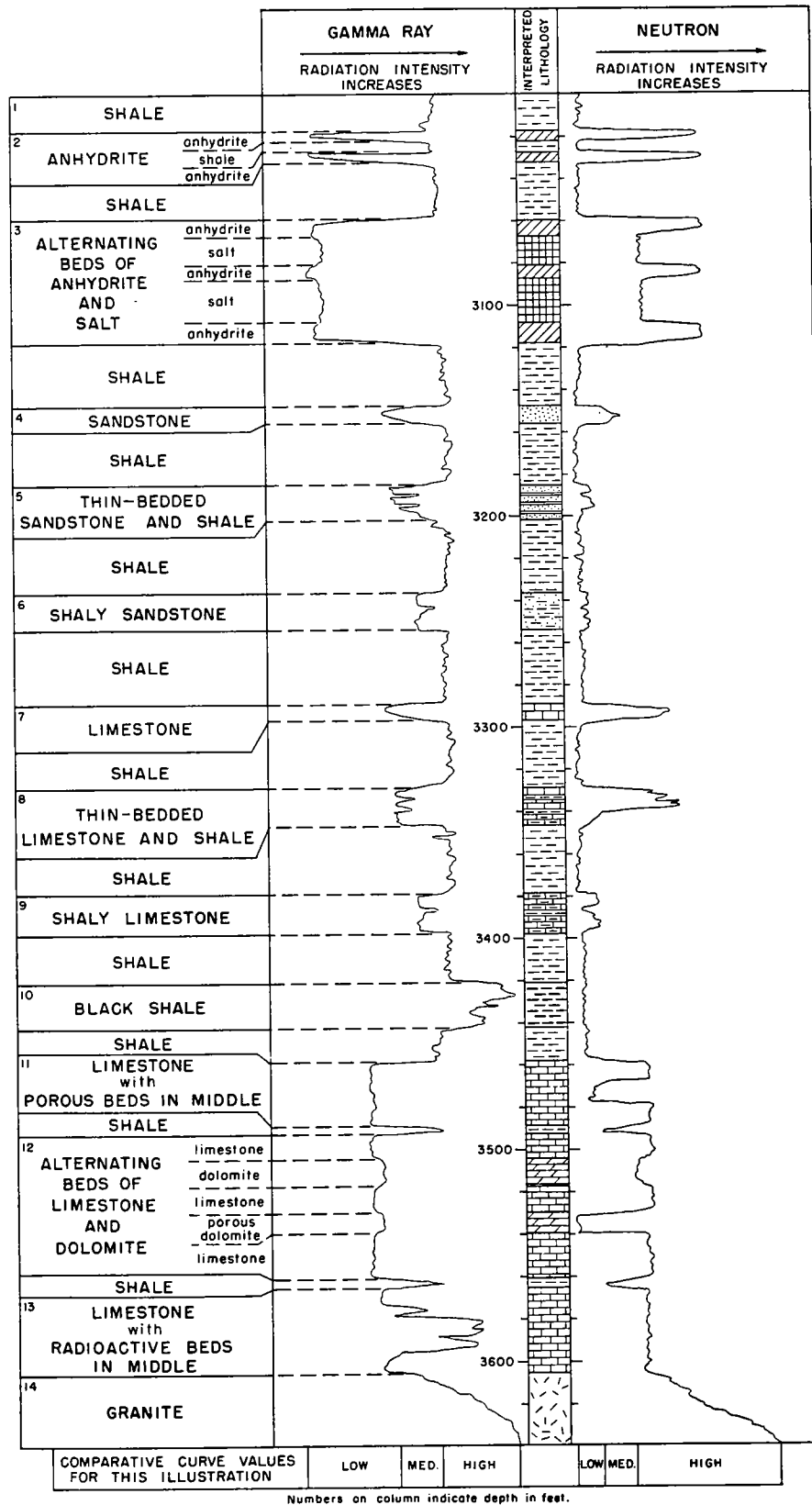
Fig. 4.- Radioactivity-log curves and their characteristic expression of common lithologies. (Adapted from Lane-Wells manual, "Radioactivity well logging.")
