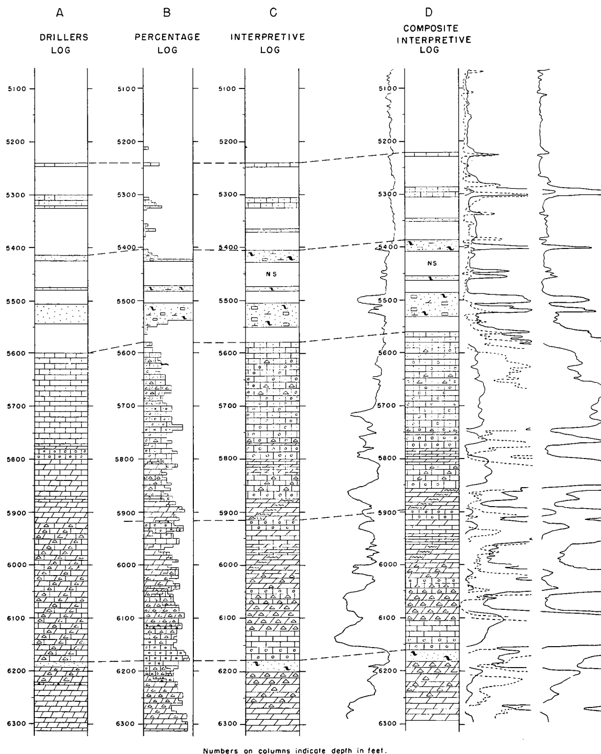
Fig. 7.- Comparison of drillers log (A), percentage log (B), interpretive log (C), and composite interpretive log (D), of same well. Electric-log curves have been added to (D) to indicate method of correcting log for sample lag. Identical beds have been logged about 20 feet higher in (D) than in (A), (B), or (C), as indicated by dashed lines. (See pl. I for explanation of lithologic symbols.)
