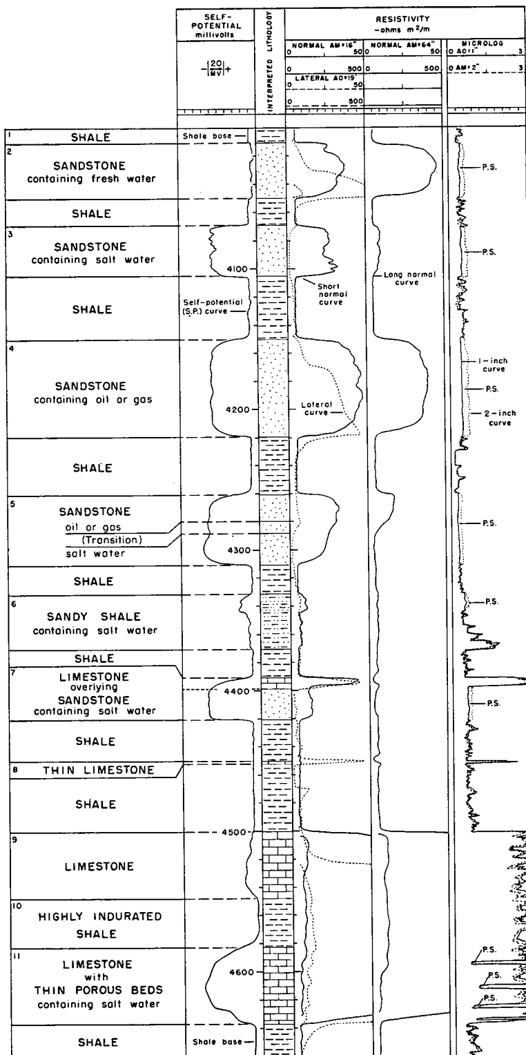
Fig. 2.- Electric-log curves and their characteristic expression of common lithologies, fluids, and gas. Dolomite, anhydrite, and quartzite record curves similar to those shown for limestone. Permeable beds are indicated by positive separations (P.S.) of micro-resistivity curves. (Adapted from unpublished diagrams of C.K. Ruddick, Schlumberger Well Surveying Corporation, Tulsa, Oklahoma.)
