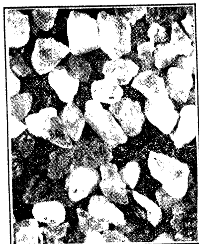
B. Medium sand (1/4-1/2mm.), x 18
