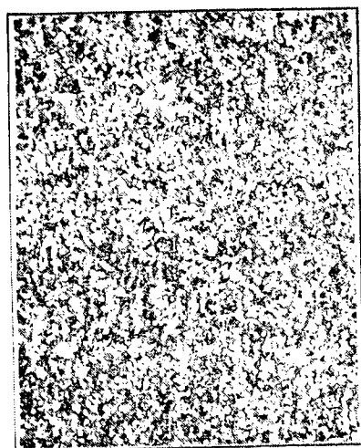
E. Very fine sand (1/16-1/8 mm.), x 6.3
