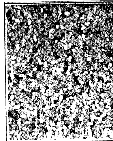
D. Fine sand (1/8-1/4 mm.), x 6.3
