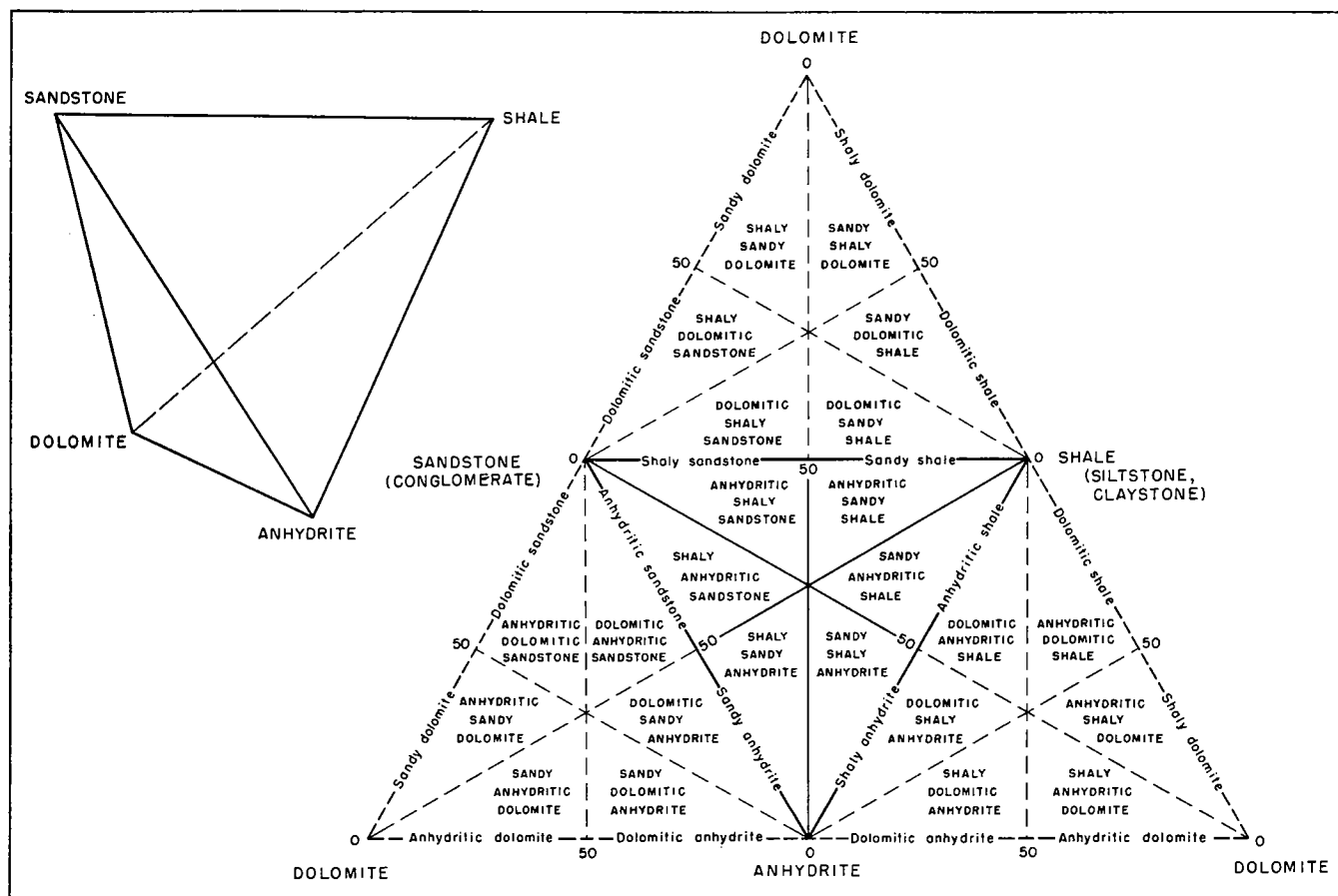
Fig. 12.— Tetrahedral diagram illustrating classification of commonly associated evaporite and siliceous clastic rocks in drill cuttings.
