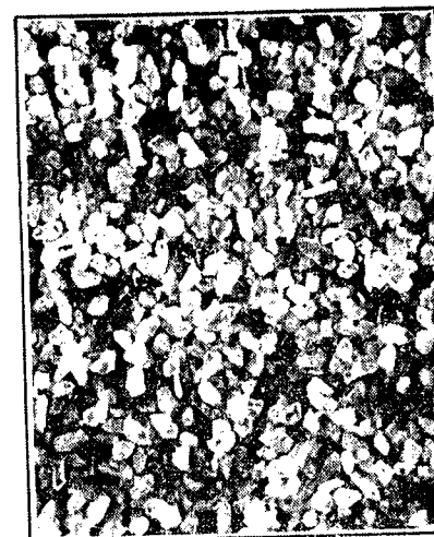
D. Very fine sand (1/16-1/8mm.), x 18
