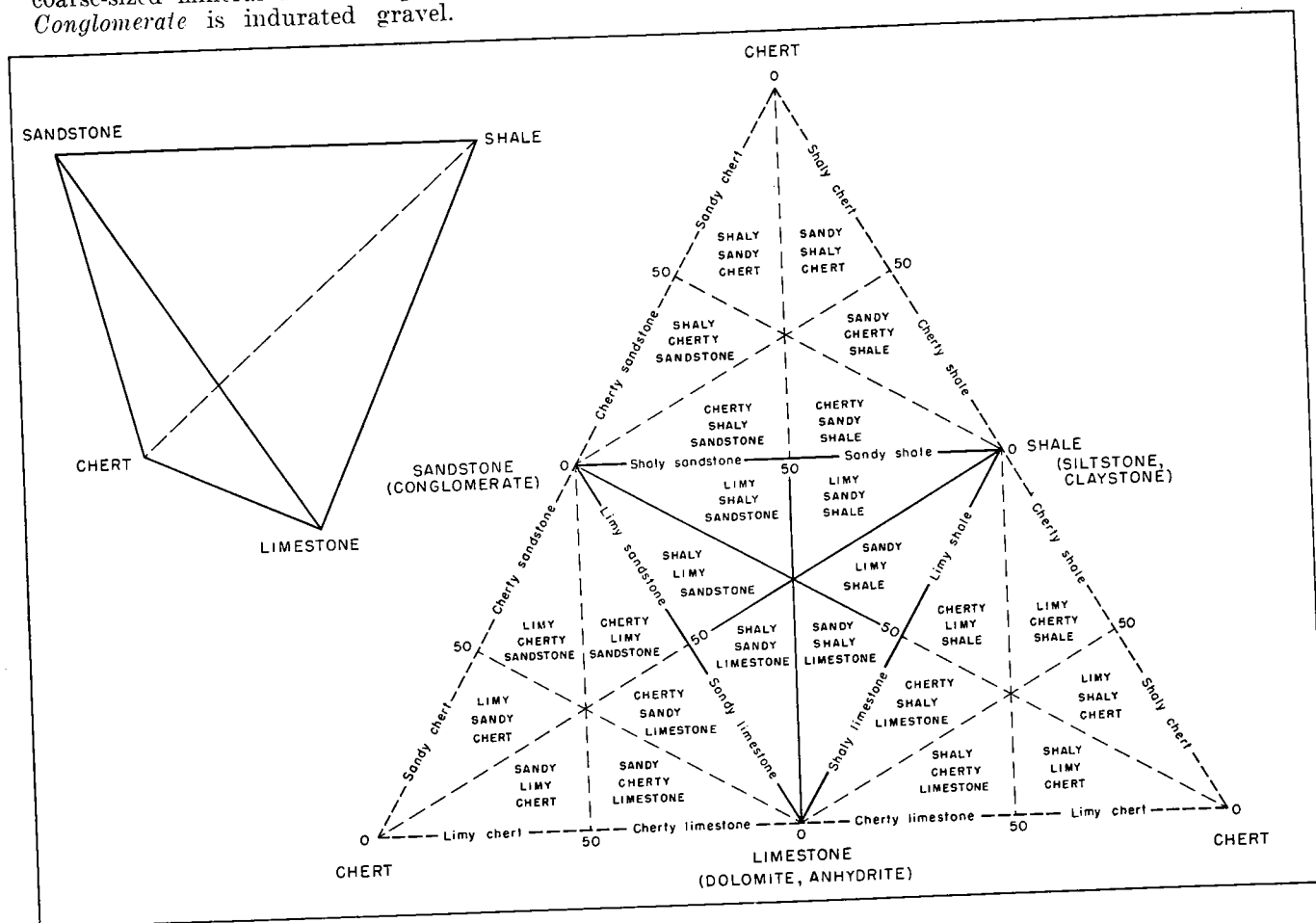
Fig. 13.— Tetrahedral diagram illustrating classification of commonly associated precipitate and siliceous clastic rocks in drill cuttings.
