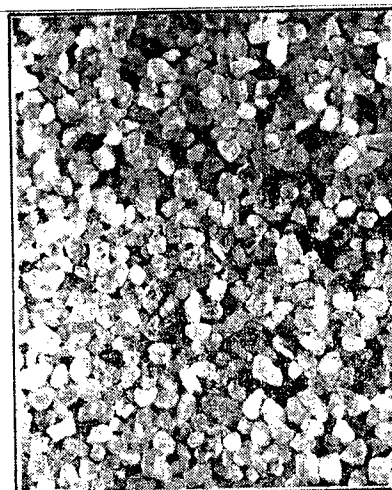
C. Medium sand (1/4-1/2 mm.), x 6.3
