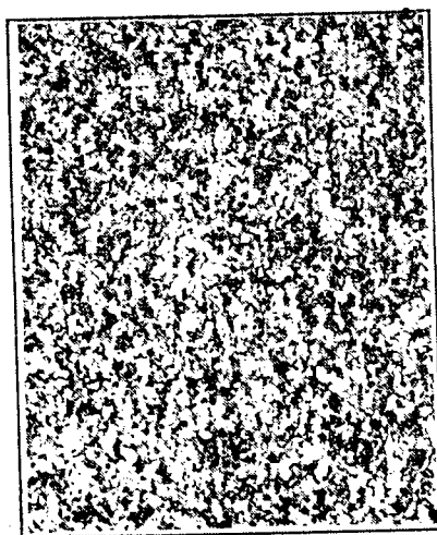
E. Unsorted silt (1/16-1/256 mm.), x 18
