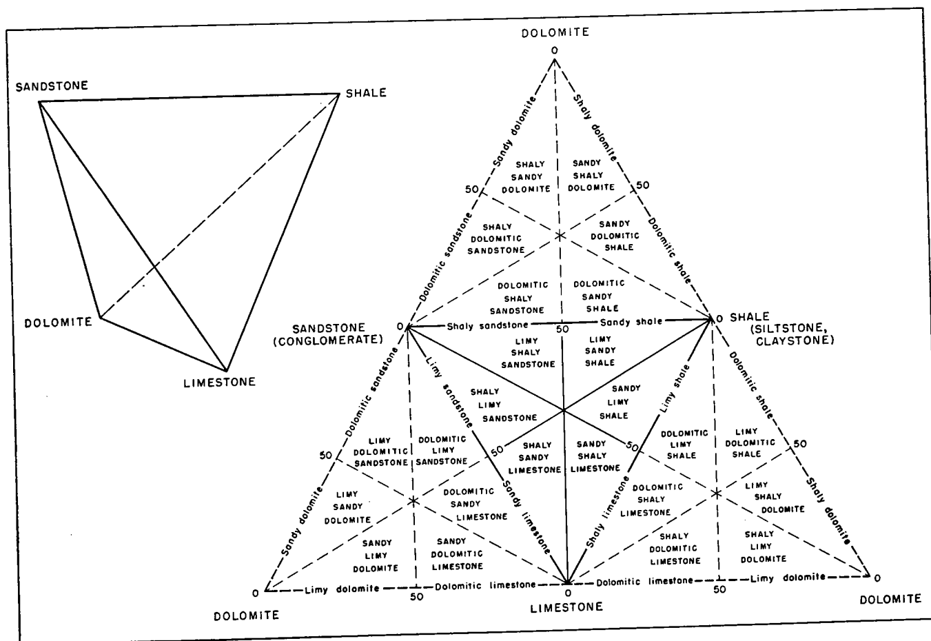
Fig. 11. — Tetrahedral diagram illustrating classification of commonly associated carbonate and siliceous clastic rocks in drill cuttings.
