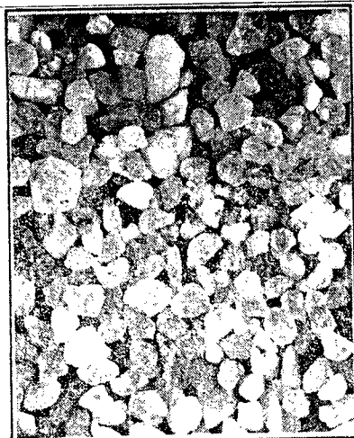
B. Coarse sand (1/2-1 mm.), x 6.3
