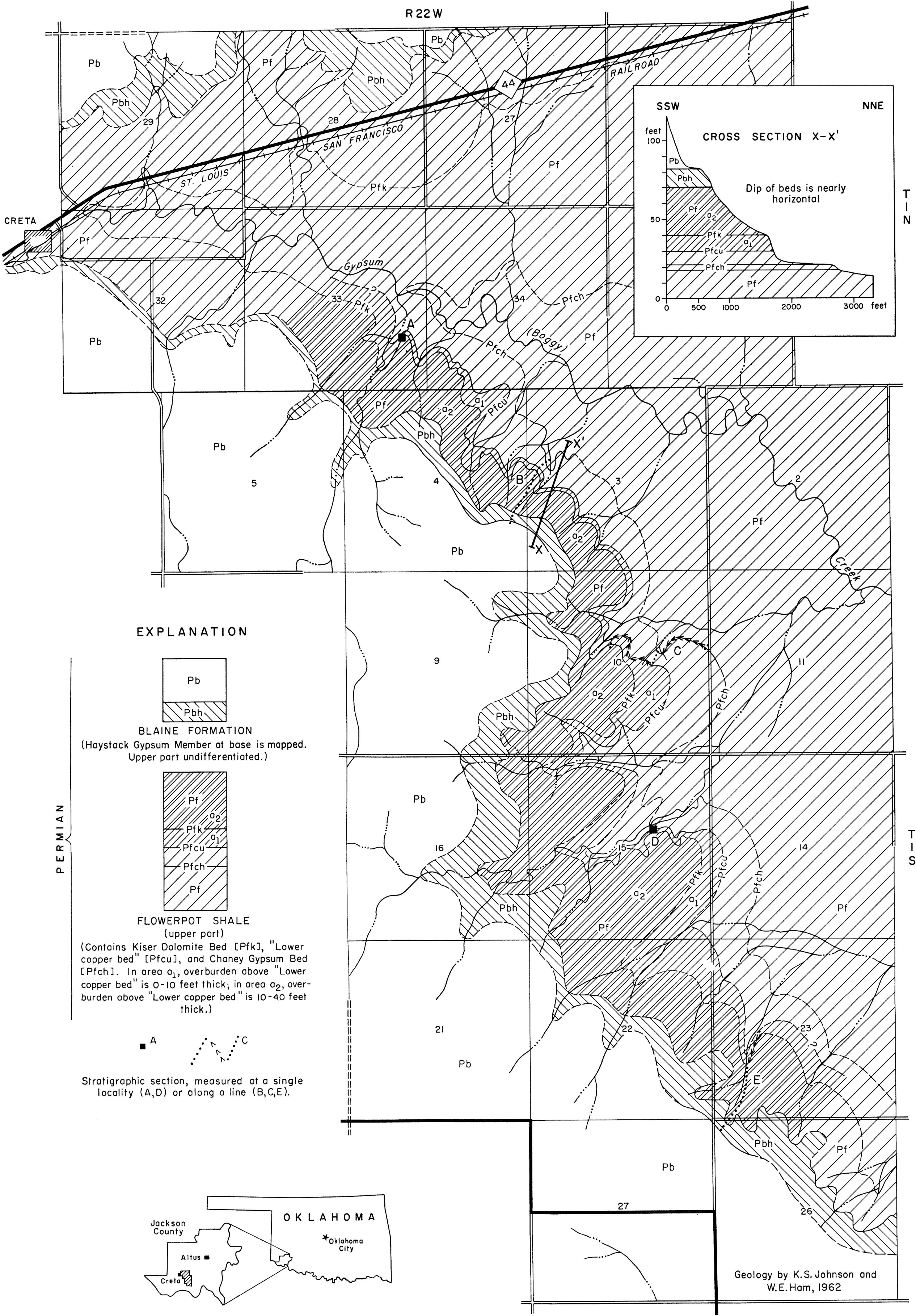
GEOLOGIC MAP OF FLOWERPOT SHALE IN THE CRETA AREA JACKSON COUNTY, OKLAHOMA
