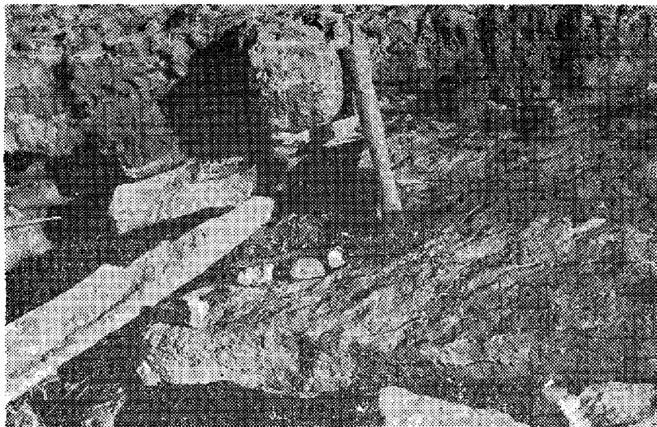
FIG. 10. Webbers Falls calcarenite grading upward into siltstone at position of tip of hammer handle. Near C. N. L. sec. 34, T. 16 N., R 19 E, Cherokee County, Oklahoma. This former exposure is now beneath the water of Fort Gibson Lake, near the eastern shore.
