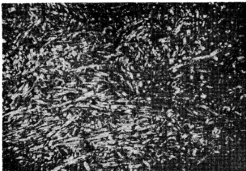
FIG. 18. Thin section of Webbers Falls chert showing matted and interwoven spicules (X 25). SE \frac{1}{4} sec. 7, T. 17 N., R. 19 E., Wagoner County, Oklahoma.
