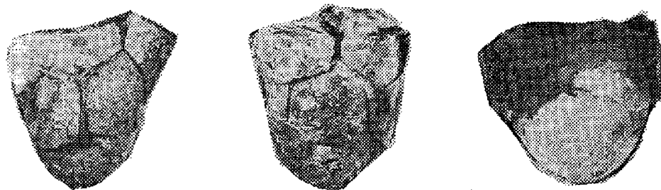
FIG. 24. Paragassizocrinus new species. Two views of the most complete calyx, view of a basal cup.
