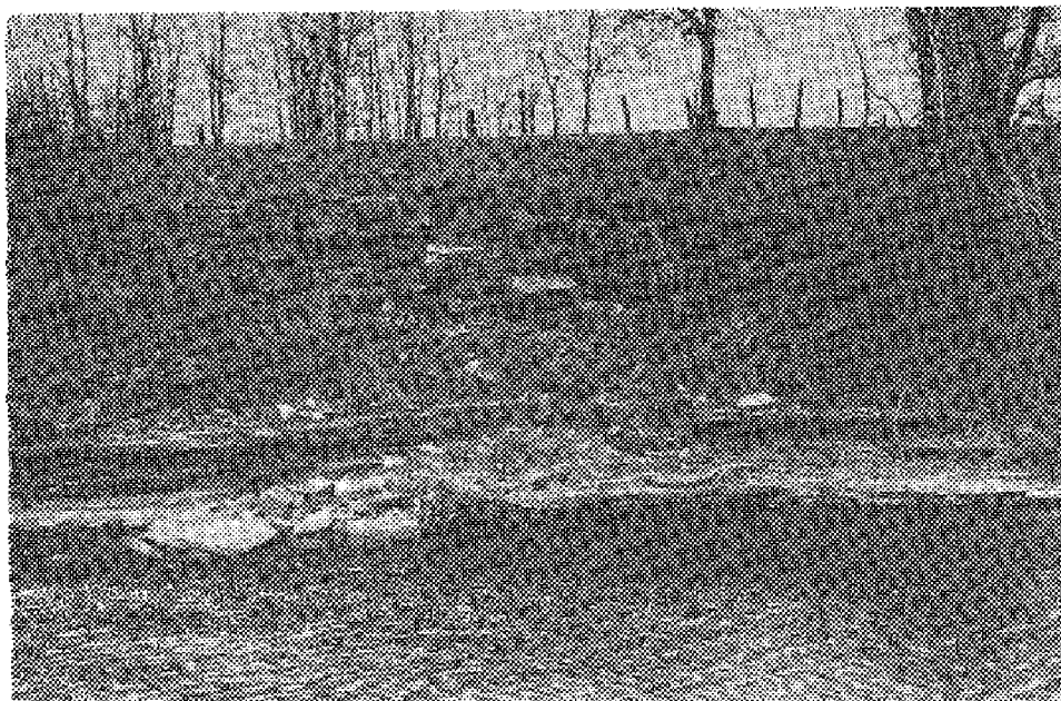
FIG. 13. Webbers Falls siltstones, limestones, and shales at Hulbert Landing, SW \frac{1}{4} sec. 21, T. 17 N., R. 20 E., Cherokee County, Oklahoma.
