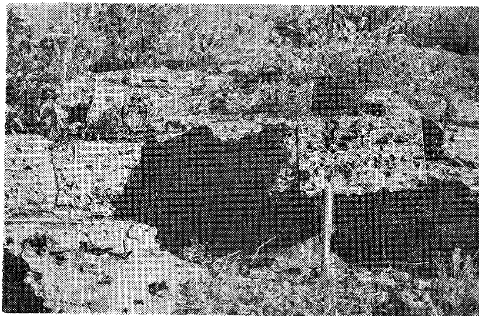
FIG. 7. Cavernous Webbers Falls siltstone, exhibiting characteristic "termite-riddled" appearance. Near C. N. L. sec. 34, T. 16 N., R. 19 E., Cherokee County, Oklahoma. This former exposure is now beneath the water near the eastern shore of Fort Gibson Lake.
