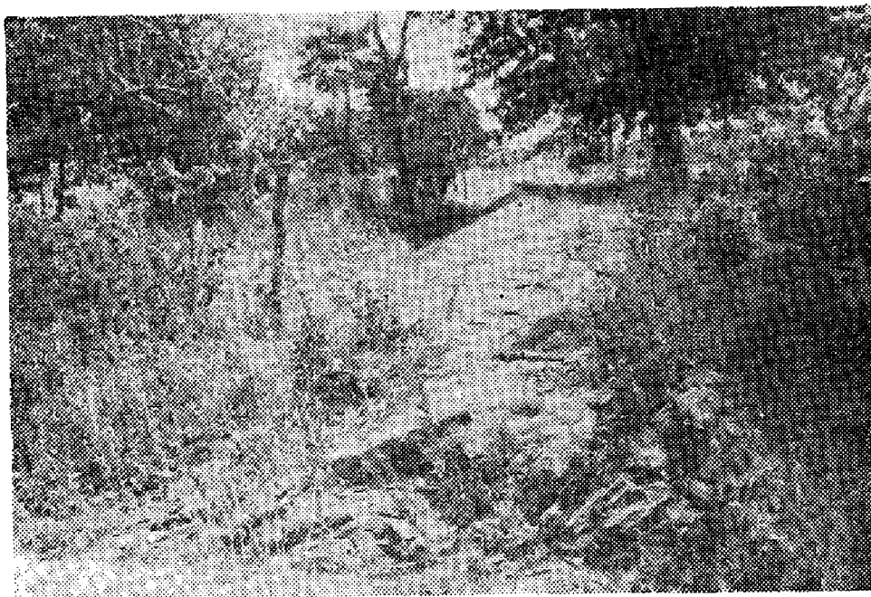
FIG. 6. Lower Atoka sandstone resembling the Pope Chapel facies. Steep dip is drag near northern fault of the Seneca graben. SW \frac{1}{4} SW \frac{1}{4} sec. 15, T. 22 N., R. 20 E., Mayes County, Oklahoma.
