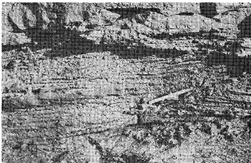
FIG. 11. Calcarenite portion of Webbers Falls member. Note small thrust fault or slumpage surface along line indicated by pencil. Shale chips are included in the calcarenite. Near C. N. L. sec. 34, T. 16 N., R. 19 E., Cherokee County, Oklahoma. This former exposure is now beneath the water of Fort Gibson Lake.
