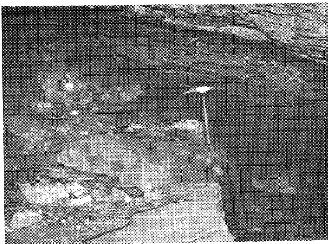
FIG. 2. View of the disconformable contact between the overlying Atoka channel conglomerate and the underlying Morrow (Hale) calcarenite, NW \frac{1}{4} sec. 20, T. 18 N., R. 19 E., on the western shore of Fort Gibson Lake, Wagoner County, Oklahoma. Hammer head is in contact with one of the ocherous clay pods which are abundant in the basal portion of the conglomerate; the end of the handle rests upon the Hale calcarenite.
