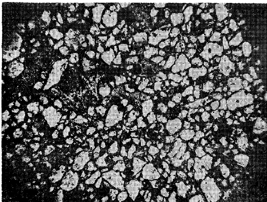
FIG. 17. Thin section of Pope Chapel sandstone, showing subangular quartz grains, many of which contain inclusions. SE \frac{1}{4} sec. 34, T. 15 N., R. 19 E., Muskogee County, Oklahoma. (X 25).
