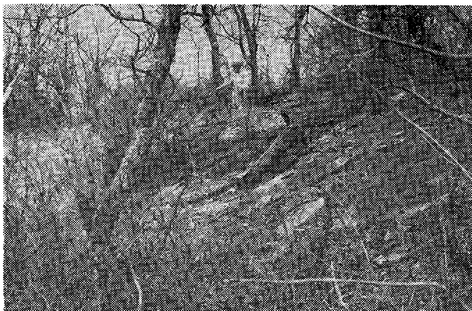
FIG. 22. Steeply dipping Morrow limestone involved in the zone of drag along a northwest-southeast fault in SW \frac{1}{4} sec. 16, T. 19 N., R. 19 E., Mayes County, Oklahoma.
