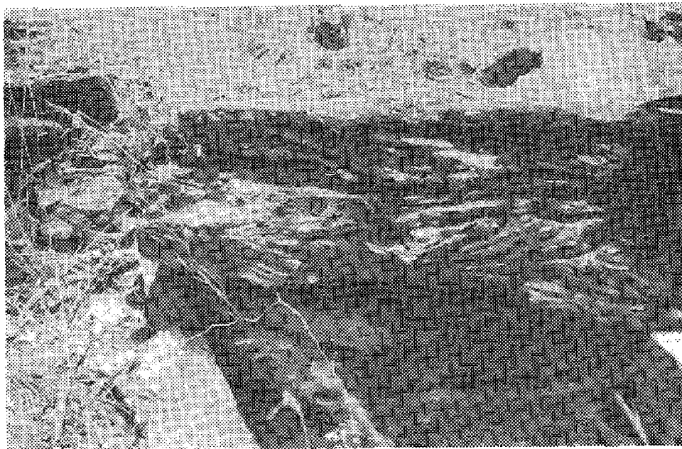
FIG. 4. Cross-bedded sandstone of the Coody-Pope Chapel sequence, NE \frac{1}{4} sec. 17, T. 18 N., R. 19 E., Wagoner County, Oklahoma.
