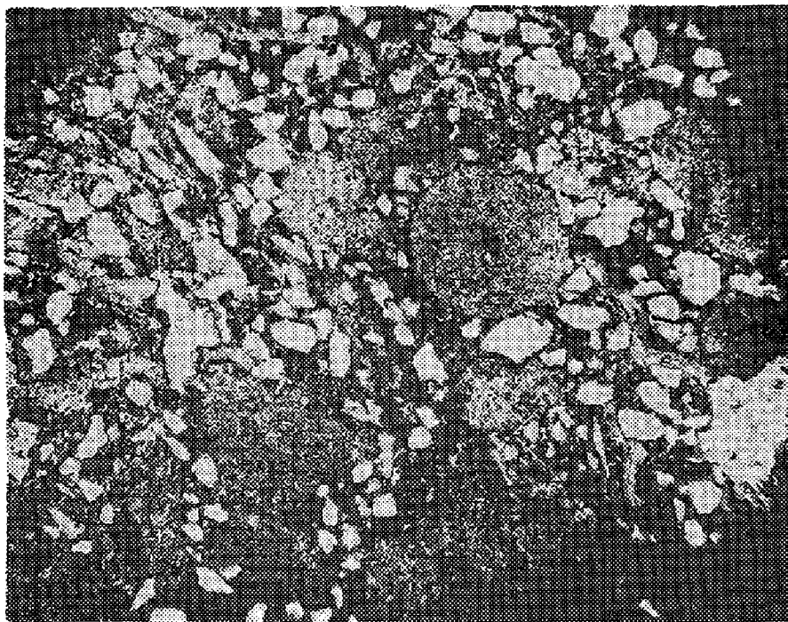
FIG. 19. Thin section of silty Webbers Falls limestone. Note echinoderm materials and angular to subangular silt particles. NW \frac{1}{4} sec. 20, T. 18 N., R. 19 E., Wagoner County, Oklahoma (X 25).
