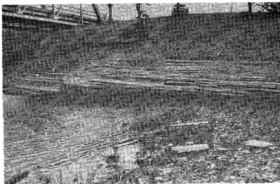
FIG. 15. Blackjack School sandstones exposed on the eastern bank of Fourteen Mile Creek, SE \frac{1}{4} sec. 21, T. 17 N., R. 20 E., Cherokee County, Oklahoma. These sandstones are thin-bedded and ripple-marked.
