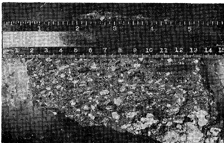
FIG. 16. Conglomeratic sandstone, presumably belonging to the Atoka formation, containing flattened pebbles of lithographic limestone derived from the underlying Fayetteville formation. Near C. E. L. sec. 21, T. 25 N., R. 21 E., Craig County, Oklahoma.
