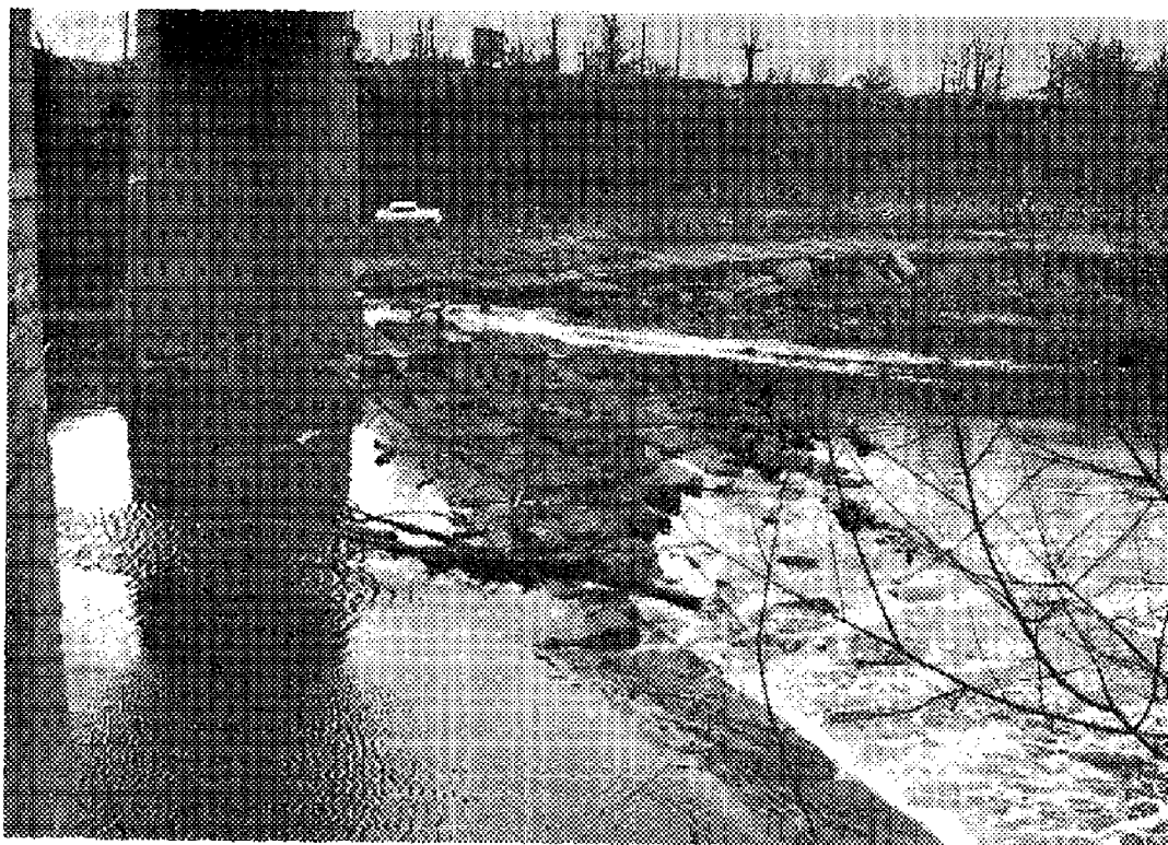
FIG. 12. Northward-dipping Webbers Falls siltstones in the bed and eastern bank of the Verdigris River at Okay, Oklahoma. The dip is believed to be due to drag along a fault which crosses the river immediately to the left of this view. Note strong regular jointing, characteristic of Webbers Falls siltstones. NE \frac{1}{4} SE \frac{1}{4} sec. 19, T. 16 N., R. 19 E., Wagoner County, Oklahoma.
