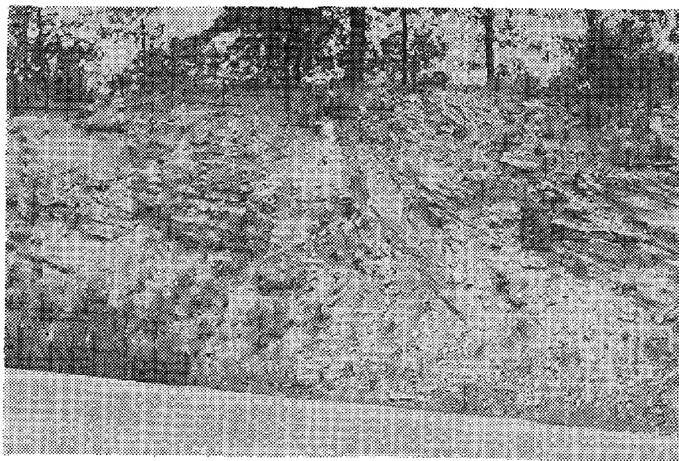
FIG. 3. Exposure of the Greasy Creek fault and the adjacent zone of drag in sandstones of the Coody member. Road cut of U. S. Highway 59, NW \frac{1}{4} sec. 5, T. 13 N., R. 25 E., Sequoyah County, Oklahoma. The left hand (south) side of the fault is the upthrown block.
