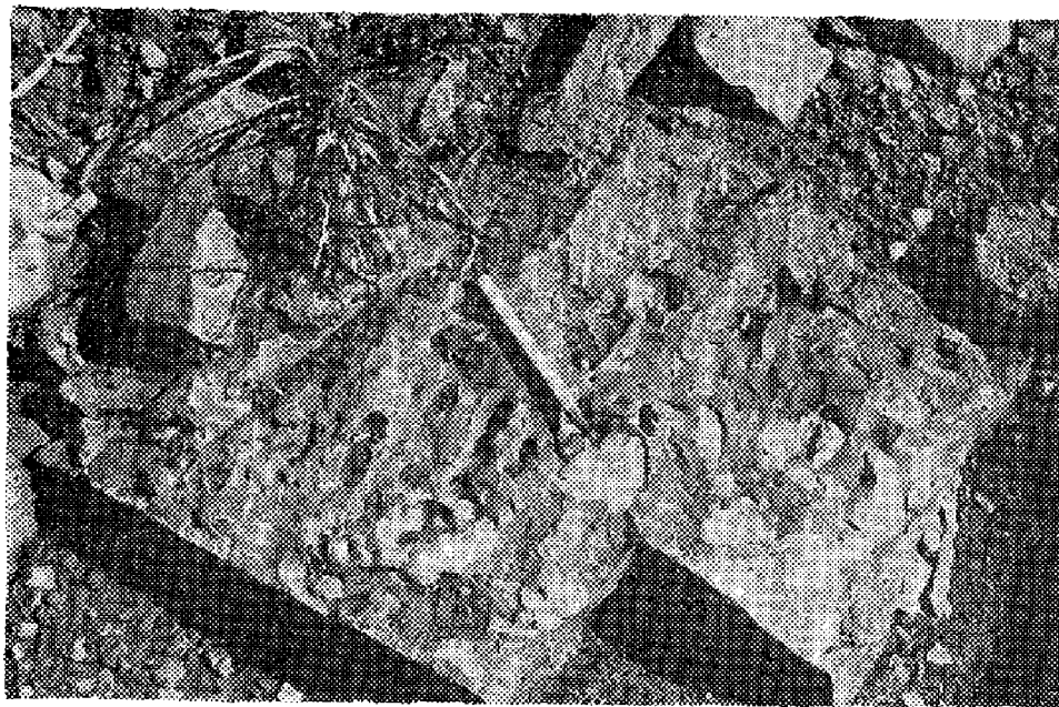
FIG. 14. Webbers Falls cavernous siltstones and core limestone. Pencil points to a localized center of limestone. Near C. N. L. sec. 34, T. 16 N., R. 19 E., Cherokee County, Oklahoma. This former exposure is now beneath the water of Fort Gibson Lake.
