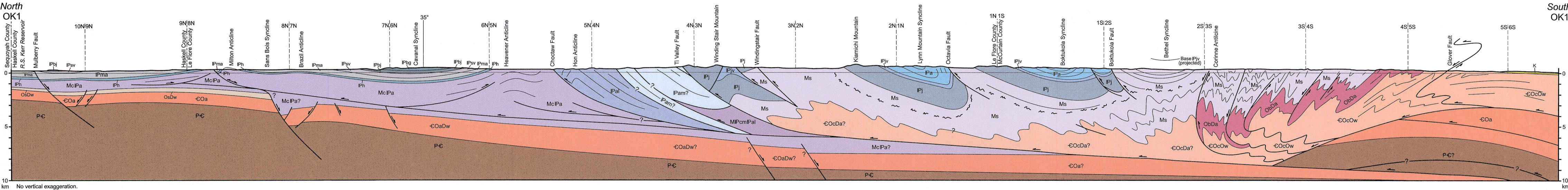
PLATE 6A STRUCTURAL CROSS SECTION OK1 ACROSS THE OKLAHOMA OUACHITA MOUNTAINS By J. Kaspar Arbenz 2008
