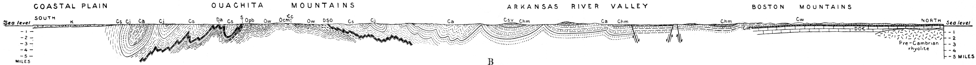
SECTION ACROSS WESTERN ARKANSAS
