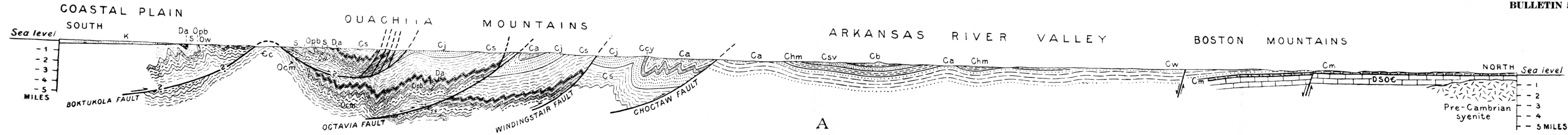
SECTION ACROSS EASTERN OKLAHOMA
