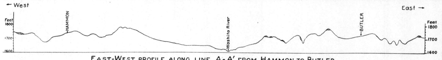
EAST-WEST PROFILE ALONG LINE A-A' FROM HAMMON TO BUTLER
