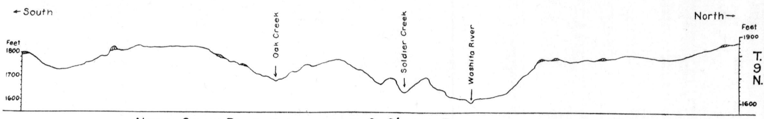
NORTH-SOUTH PROFILE ALONG LINE C-C' FROM BUTLER TO A POINT NEAR FOSS
