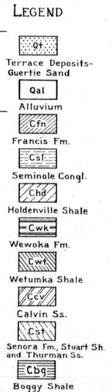
GEOLOGIC MAP OF HUGHES COUNTY BY J. PHILIP BOYLE
