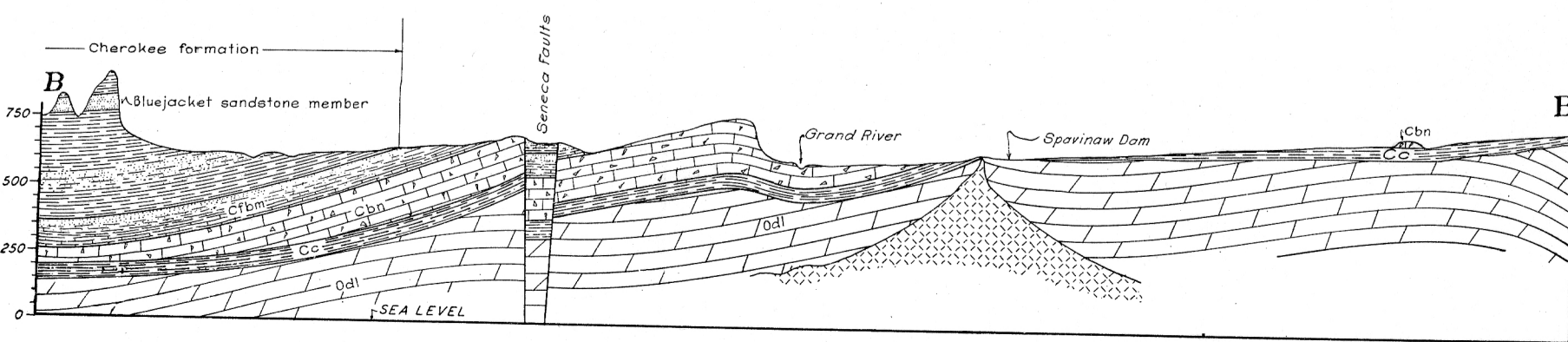
SECTION ACROSS CENTRAL MAYES AND WEST CENTRAL DELAWARE COUNTIES.
