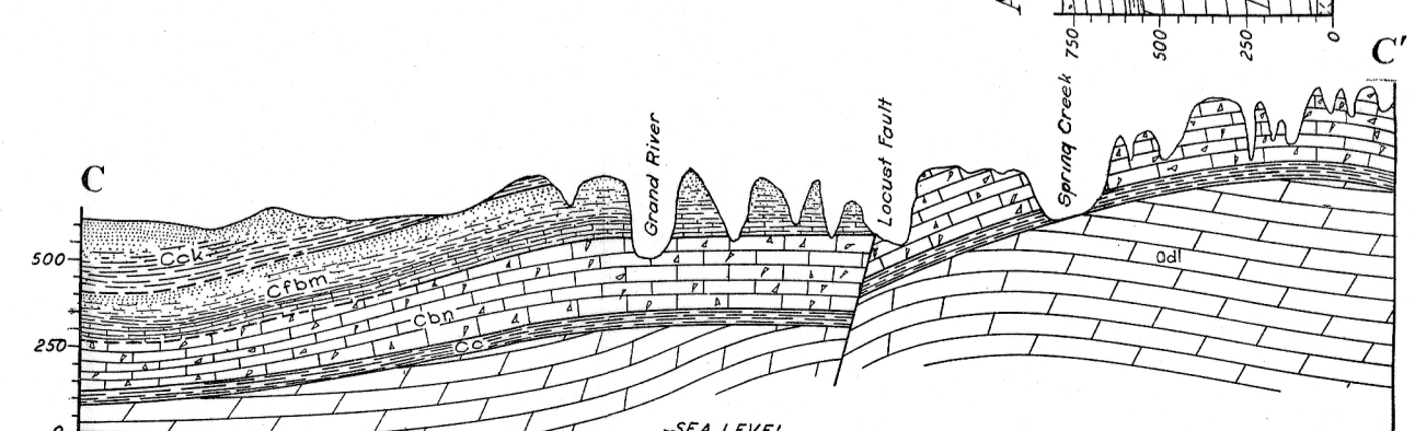
SECTION ACROSS SOUTHERN MAYES COUNTY
