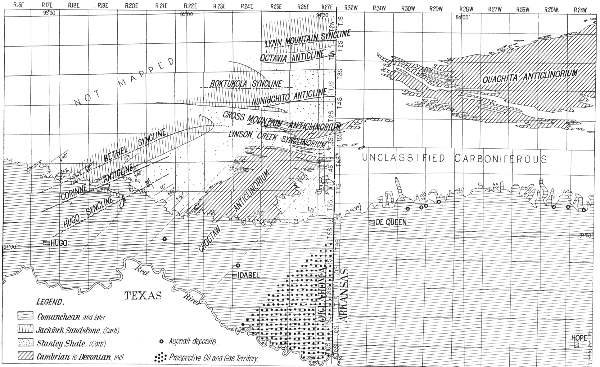
GENERAL STRUCTURAL MAP SHOWING RELATIONSHIP BETWEEN THE AREA IN SOUTHEASTERN OKLAHOMA AND THAT OF WEST CENTRAL ARKANSAS.
