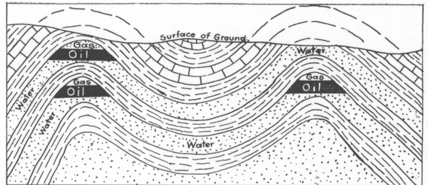
Figure 6a. Diagram representing the accumulation of oil and gas in anticlines.
