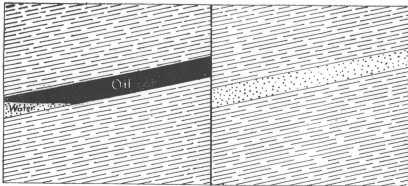
Figure 10a. Ideal section showing an oil sand faulted in such a manner that an accumulation of oil will result.
