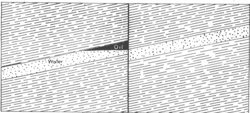
Figure 10c. Ideal section showing an oil sand faulted in such a manner that an accumulation of oil may result.
