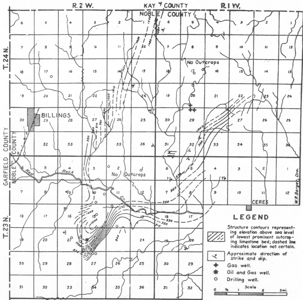
MAP OF ANTICLINAL FOLD NEAR BILLINGS, OKLAHOMA
