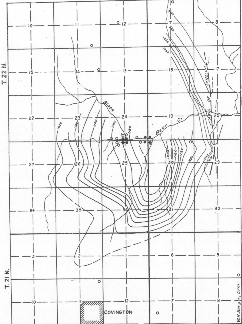
GEOLOGIC MAP OF GARBER ANTICLINE GARFIELD COUNTY, OKLAHOMA.
