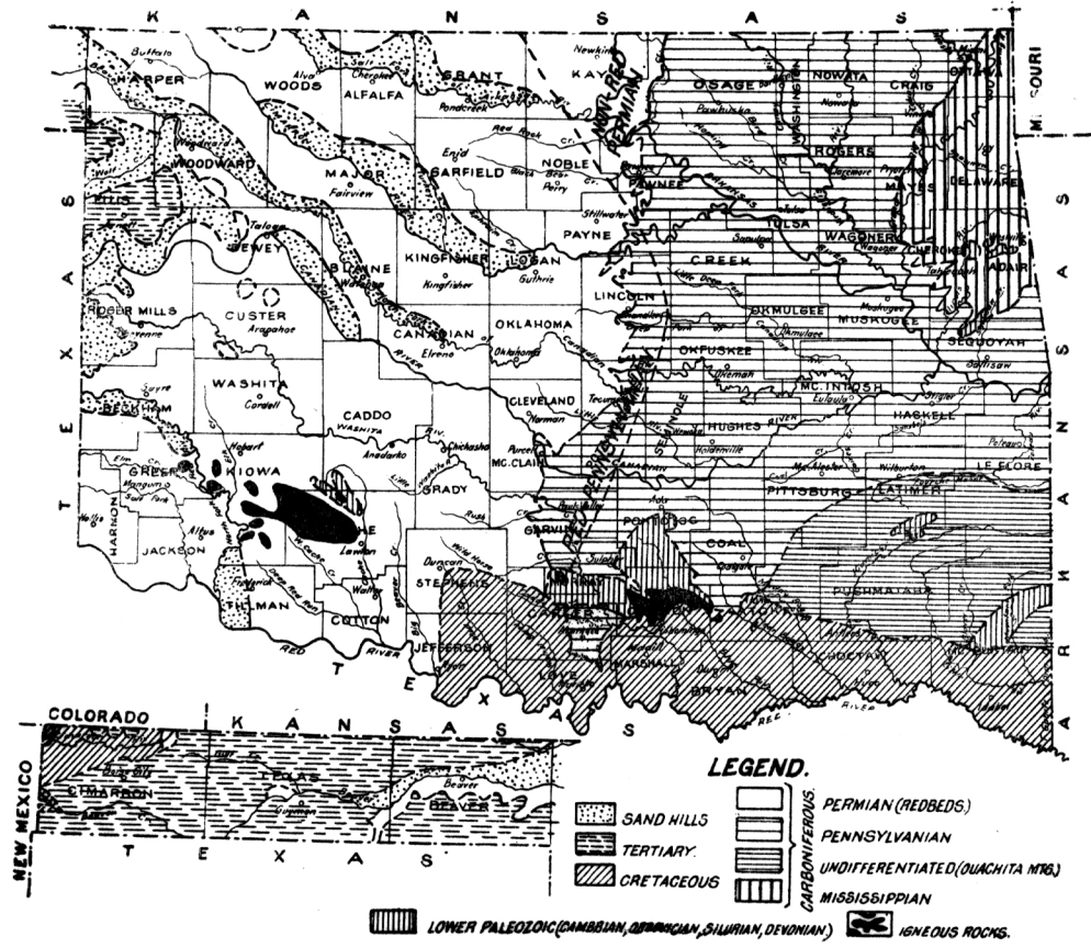
Figure 1.—GEOLOGIC MAP OF OKLAHOMA.
