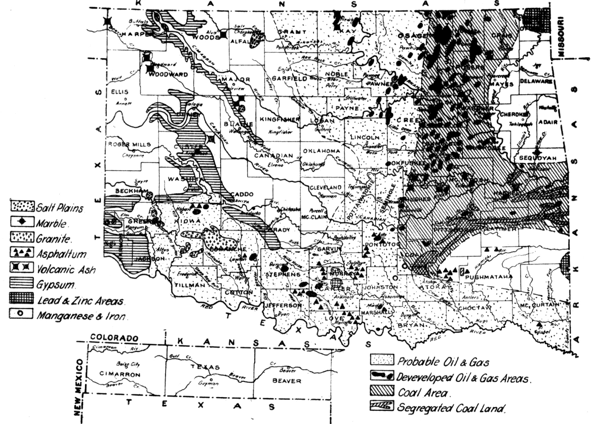
Figure 2.—MAP SHOWING DISTRIBUTION OF MINERALS IN OKLAHOMA.
