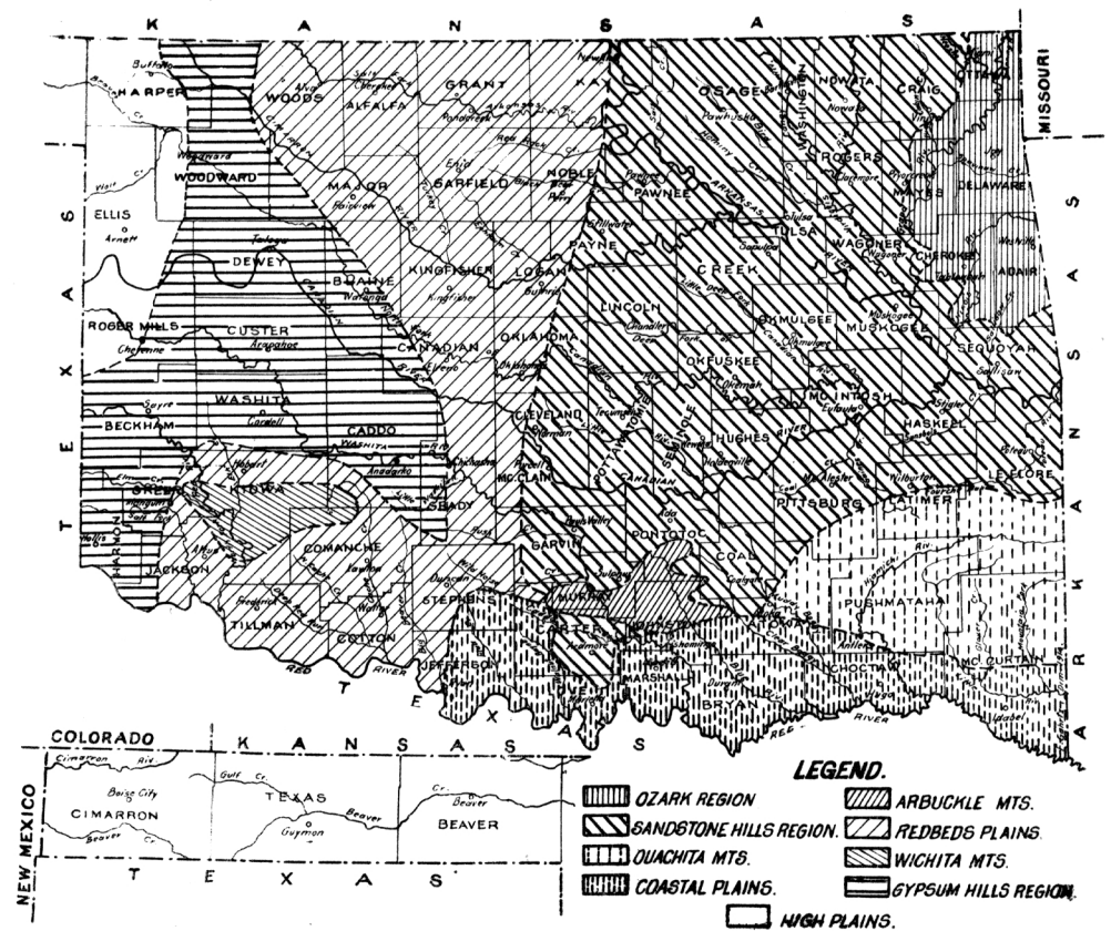
Figure 1a.—PHYSIOGRAPHIC MAP OF OKLAHOMA.
